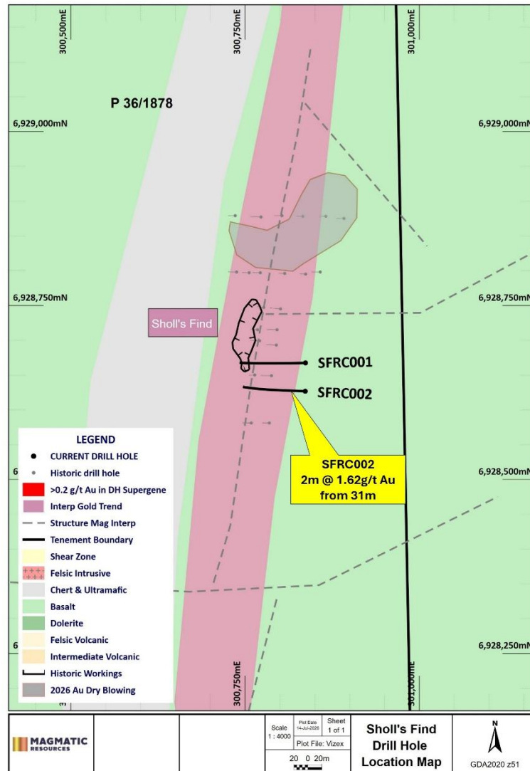
Figure 10. Sholl's Find Drill hole location plan and current drill intercepts
