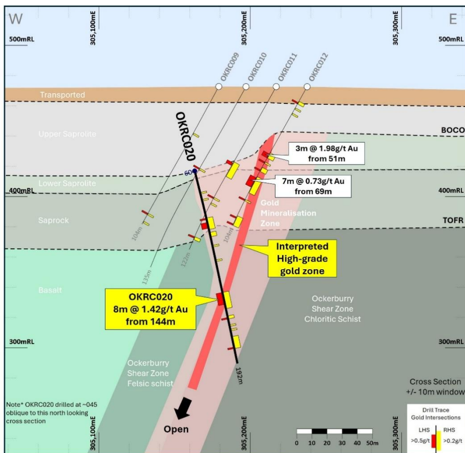
Figure 6 OKRC020 Cross Section. Ockerburry 3 Prospect. 6904280N Looking North
