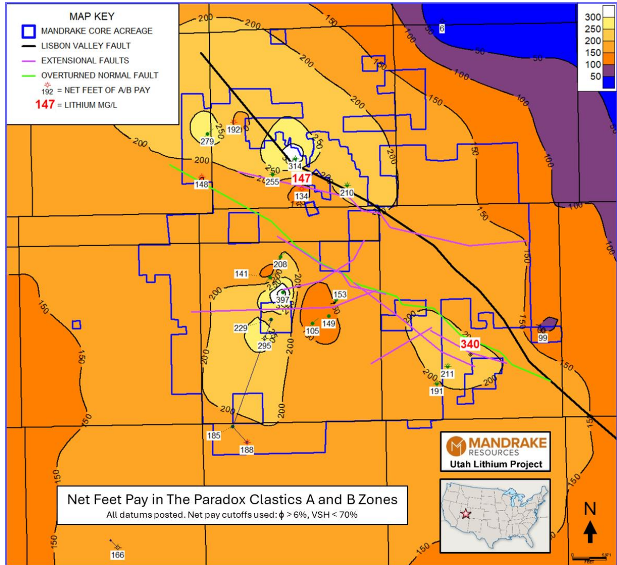
Figure 2. Net Feet Pay in the Paradox Clastics A and B Zones. Both prospective lithium samples from the Big Indian Unit #1 and the Peterson #88-21 lie in areas with faulting complexities and elevated net pay in the Paradox A/B Zones.
