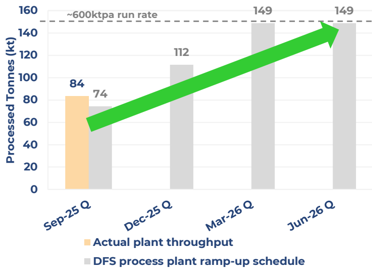
Figure 5: Ore tonnes processed.
