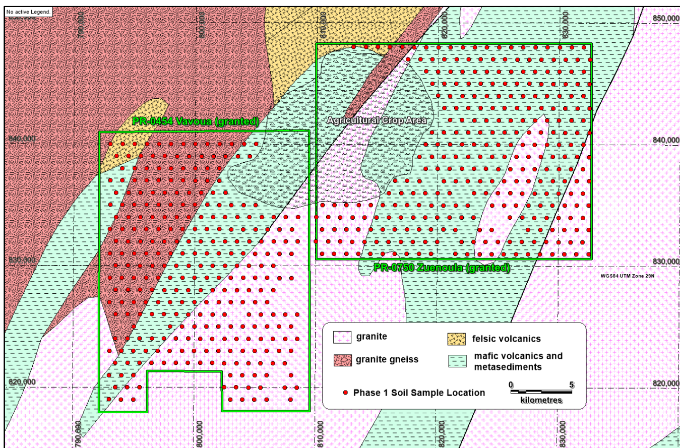
Figure 3. Map illustrating the Phase 1 soil sampling program planned for Vavoua and Zuénoula permit areas
