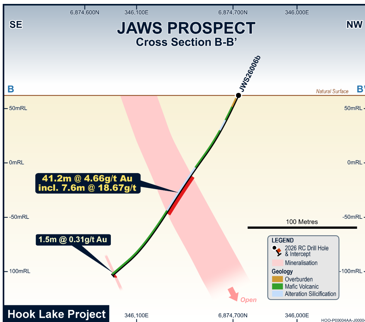
Figure 4: Drillhole section showing the location of JWS26006b without historic drillhole from the 1988 program. Mineralisation interpreted to be steeply dipping NW.
