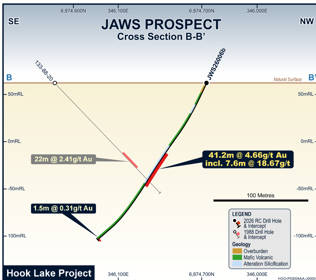
Figure 3: Drillhole section showing the location of JWS26006b compared with historic drillhole from the 1988 program. Note higher grades reported by modern drilling.
