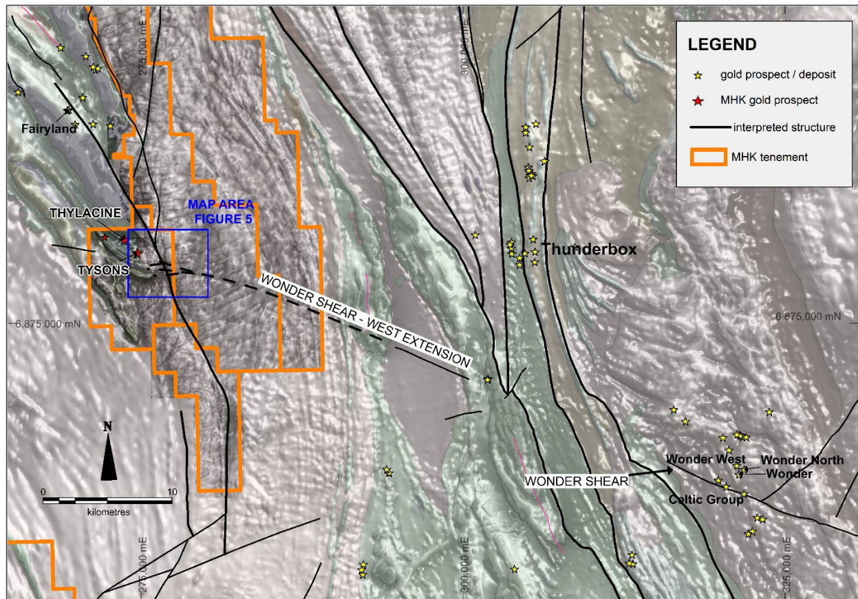
Figure 6. Leinster South tenements, regional magnetics image showing target WNW structure
