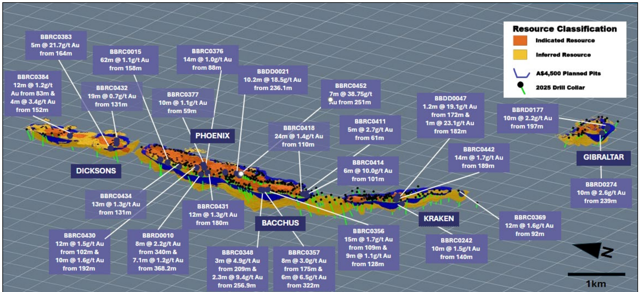
Figure 4 - Bullabulling Gold Project MRE showing key intercepts
