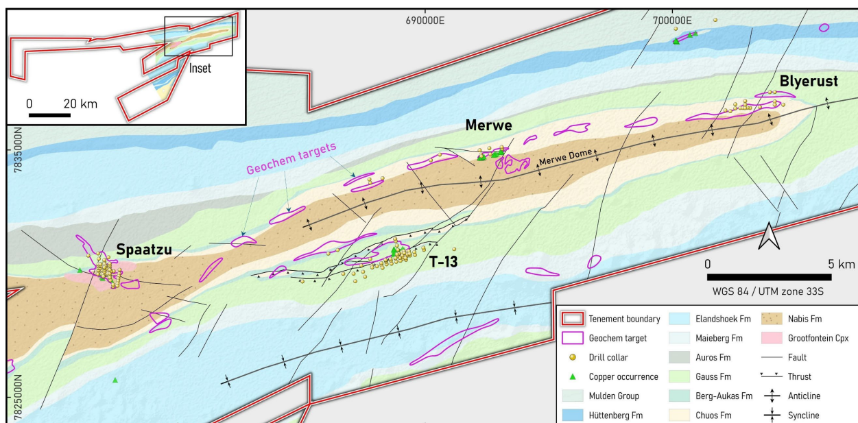
Figure 4: Location of Spaatzu and Merwe Prospects and T-13 Deposit within the Otavi Project.
