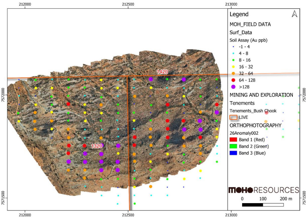
Figure 7. 2026 Anomaly 2. +32ppb gold in soil over 750m with two samples >1g/t Au
