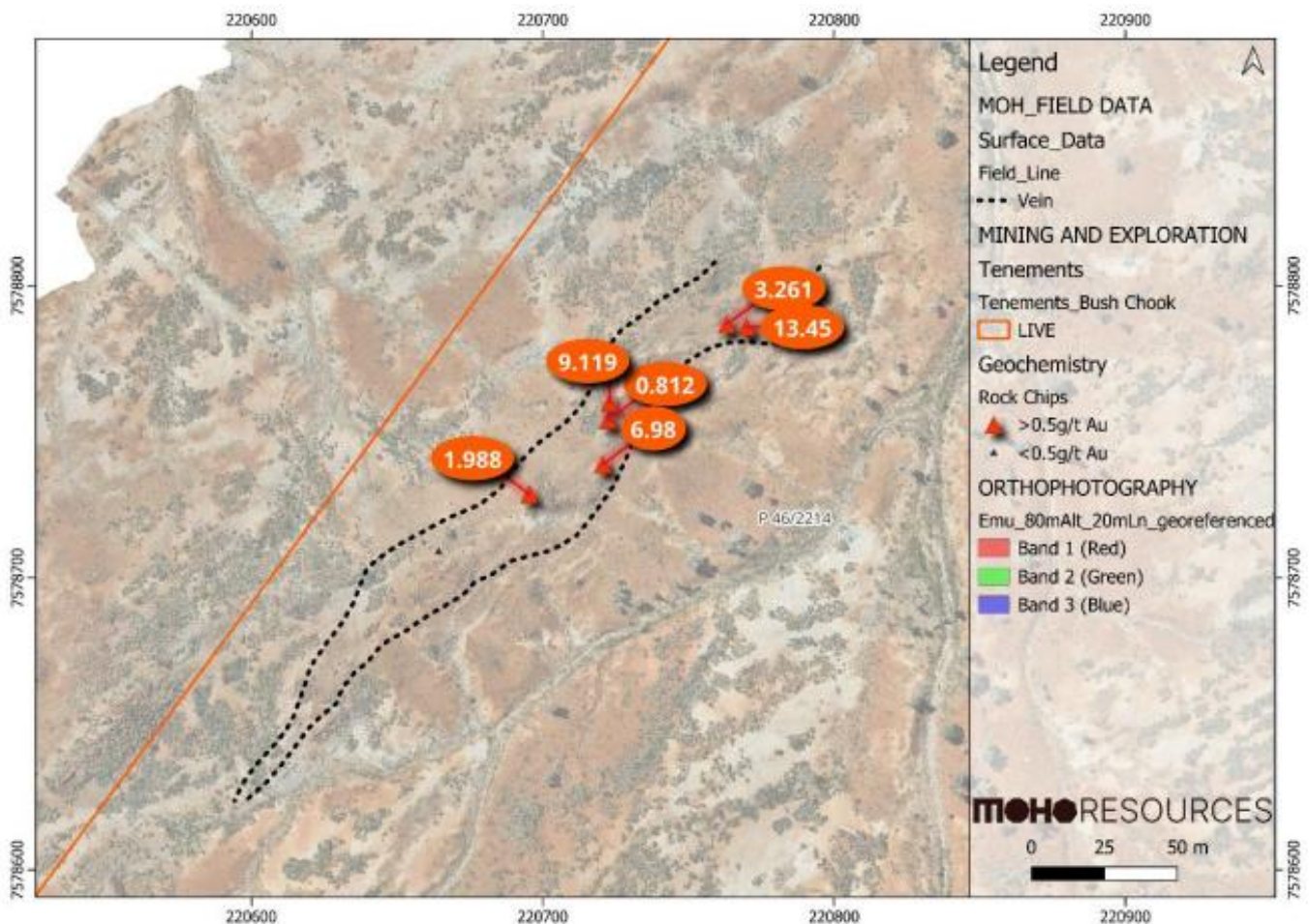
Figure 8. Emu Prospect - +100m high-grade gossanous quartz vein.
