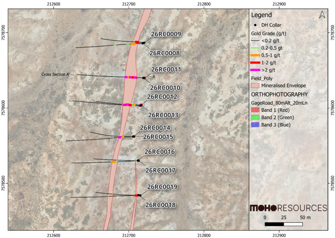
Figure 3. Gage Road Prospect drill plan
