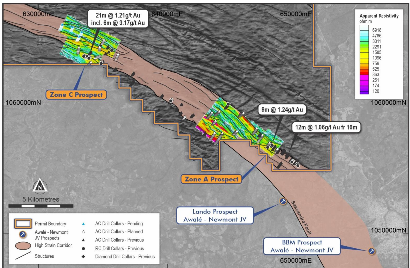
Figure 5 | Odienné Gold Project, Odienné South permit location with all drill collar and GAIP survey locations, highlighting apparent resistivity results in the GAIP survey.
