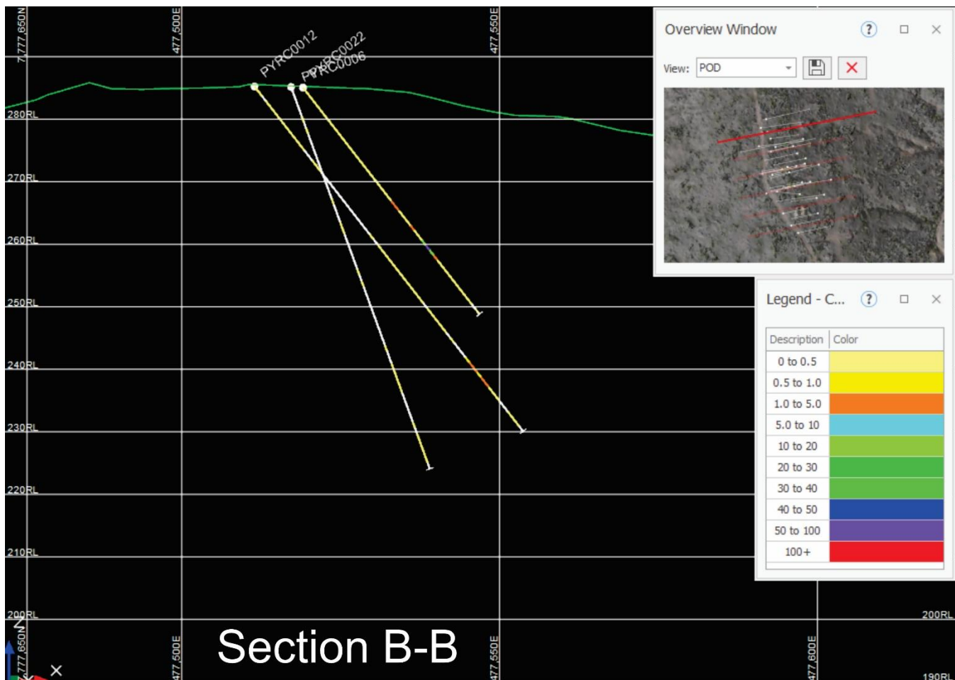
Figure 5: Section B-B
