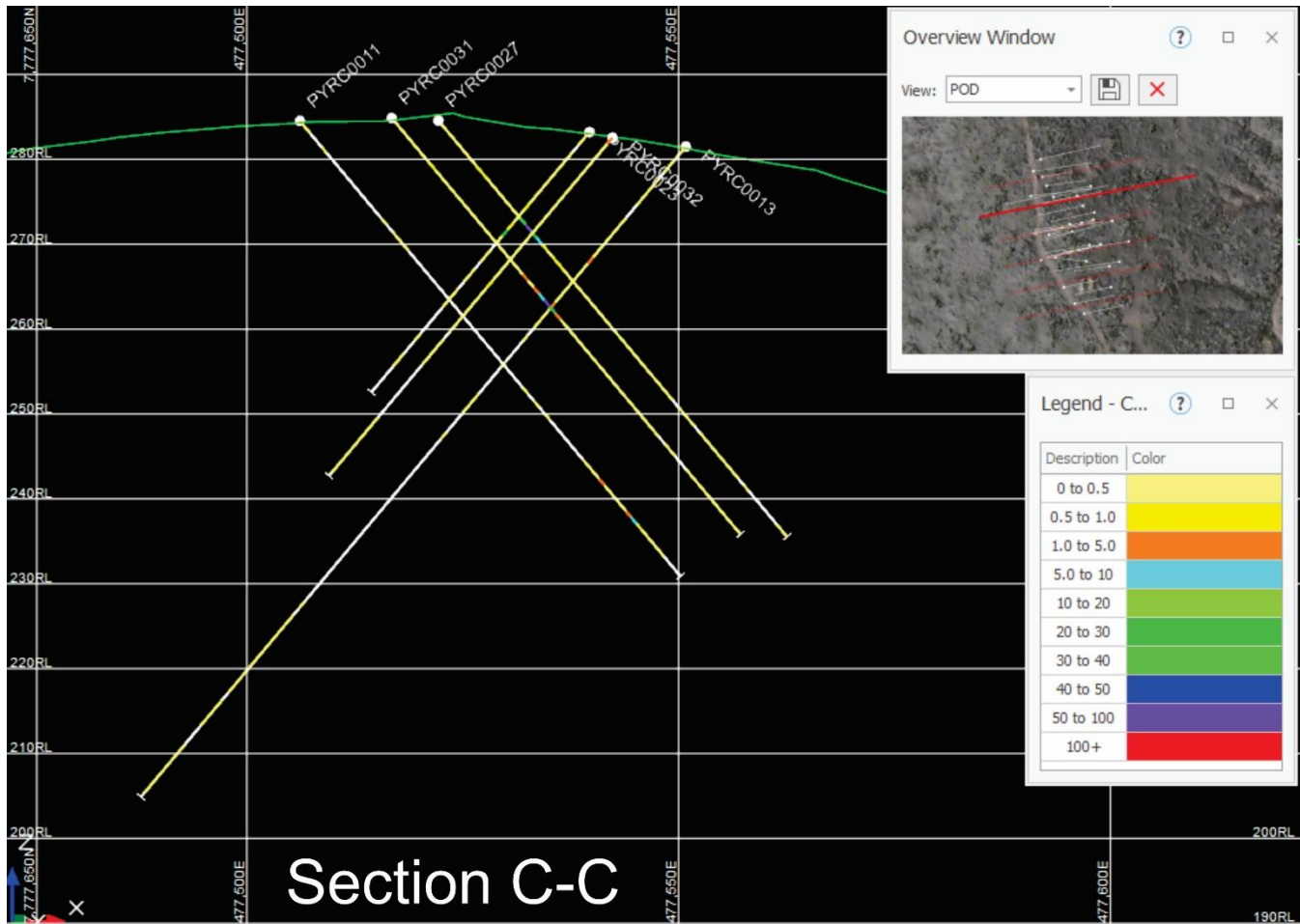
Figure 6: Section C-C
