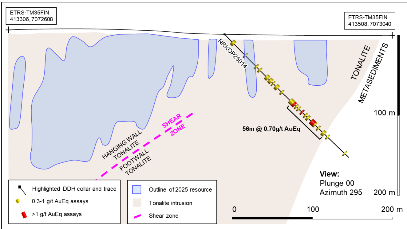
Figure 3: Kopsa section showing the drill trace for NRKOP25014. The most recent MRE outline and the interpreted extent of the tonalite intrusion are also shown in this 30m thick section view. See Appendix 1 for the drill hole details. Coordinates presented in ETRS-TM35FIN system (EPSG:3067).
