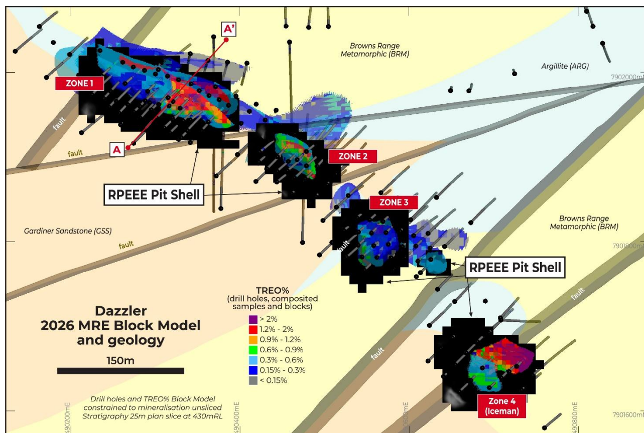
Figure 8 – Plan view of Dazzler
