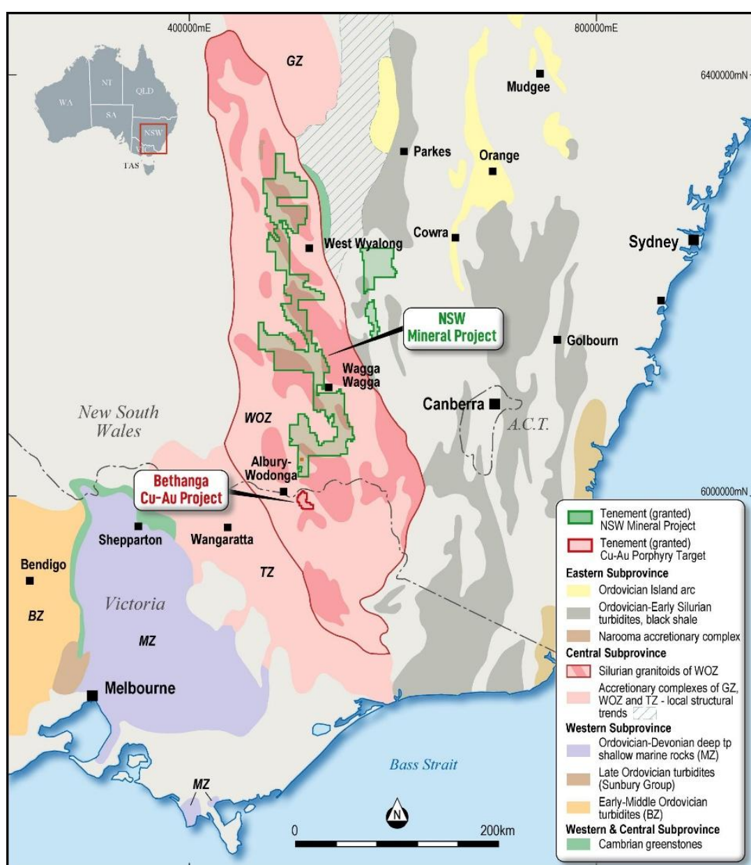
FIGURE 20: NEXUS CRITICAL MINERALS TENURE OVER GEOLOGY
