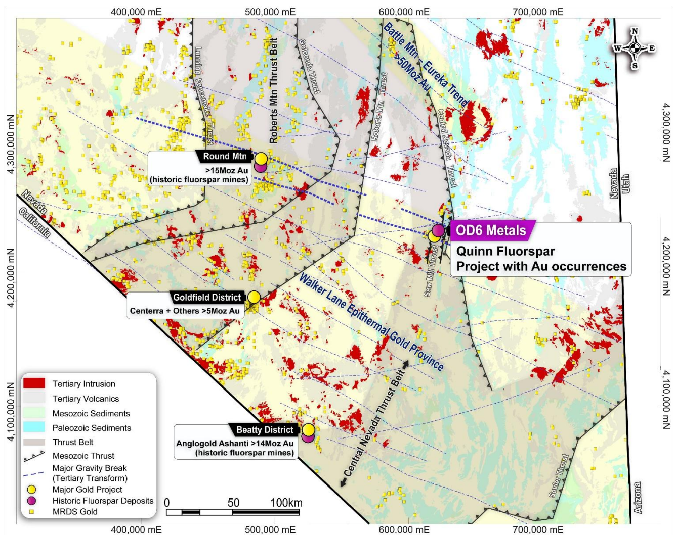
Figure 6 Regional Tertiary intrusive centres and gold deposits of the Walker Lane (Nevada BMG) with major gravity data breaks (Tertiary Transforms) and major thrusts/thrust belts (Long, 2015).
