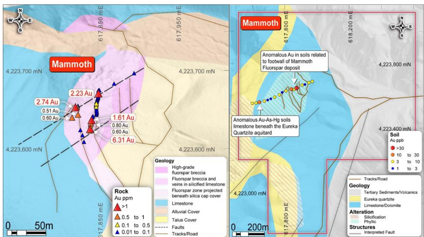
Figure 3 Left - rock chip results for Au on the Mammoth footwall. (right) gold in soils at Mammoth
