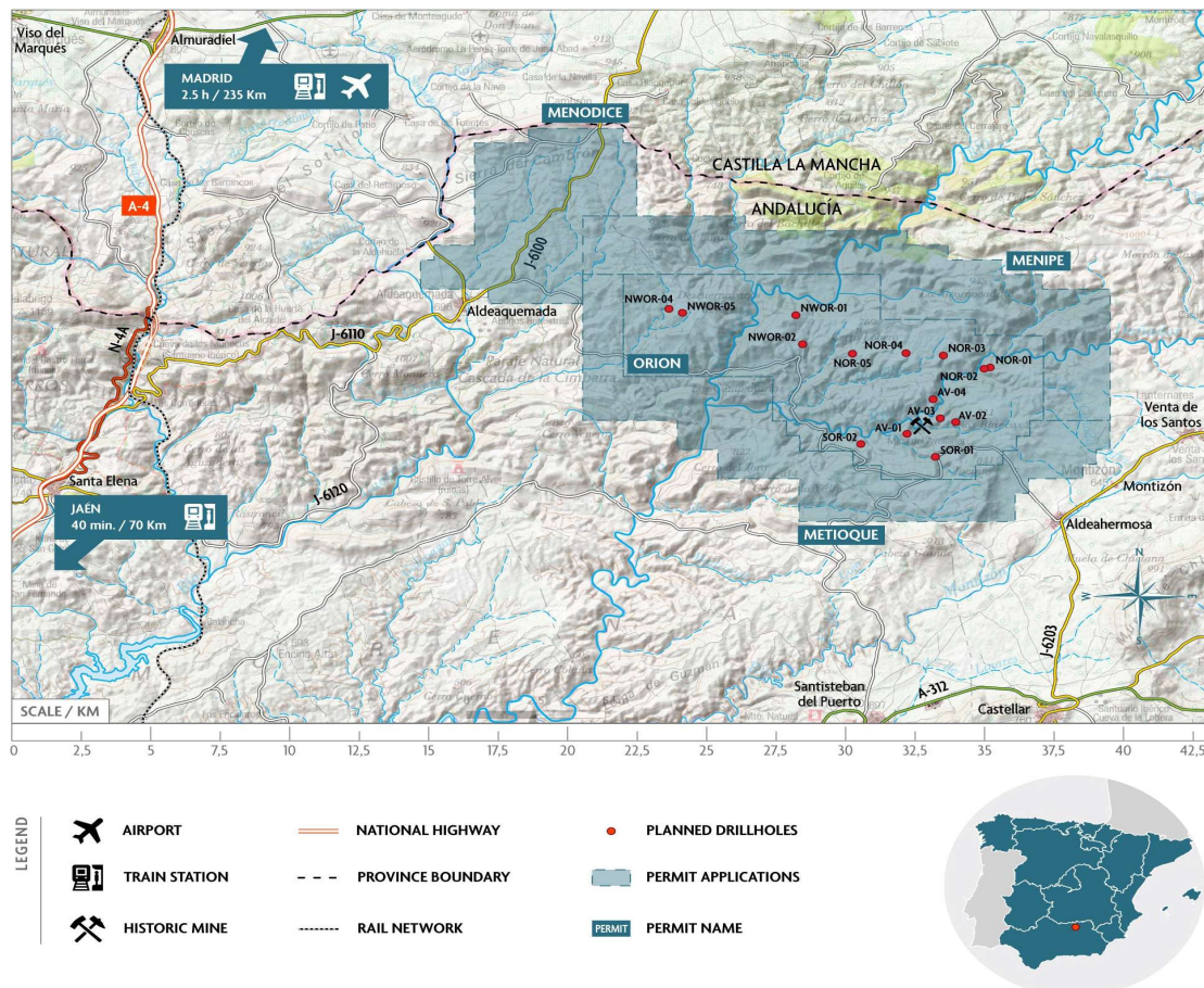
Figure 5 – Map showing Orion EU Critical Minerals Project and location of proposed drill holes.
