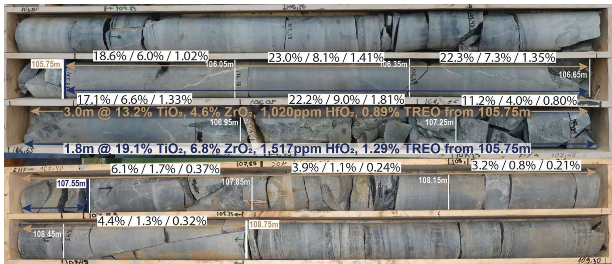
Figure 3 – Diamond drill core photos and assay data (Black: \text{TiO}_2\% / \text{ZrO}_2\% / \text{TREO}\% grades; Brown: 3% \text{TiO}_2\% cut-off weighted average grade; Blue: 8% \text{TiO}_2\% cut-off weighted average grade).
