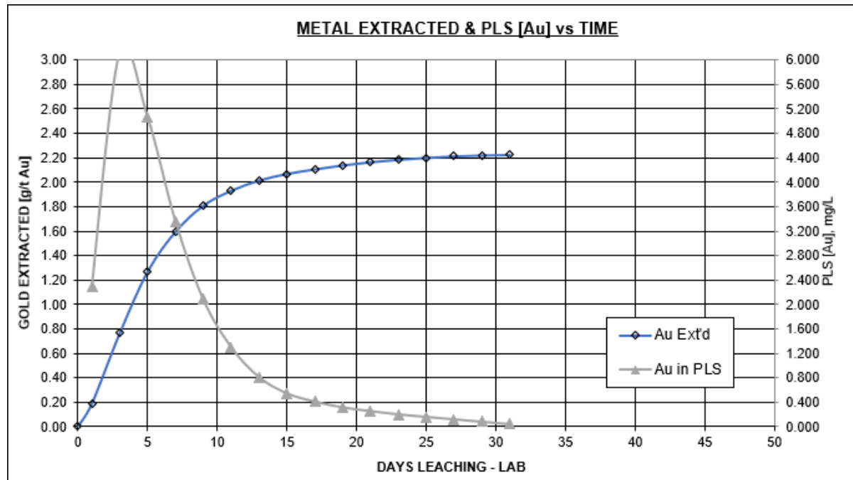
Figure 1: Gold recovered in solution (g/t Au) vs time, in days
