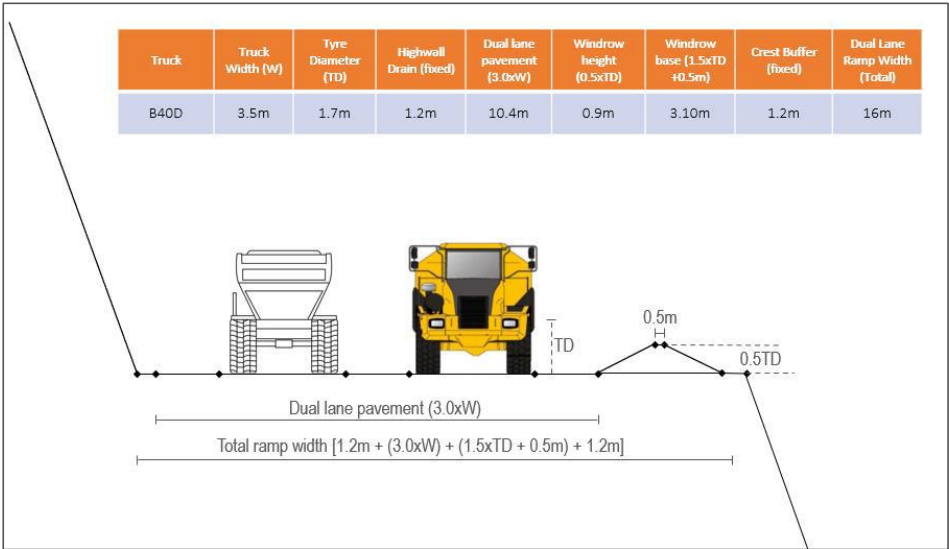
Figure 2.9: Dual lane – road width criteria
