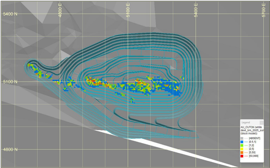
Figure 2.13: White Devil – Stage 2 pit
