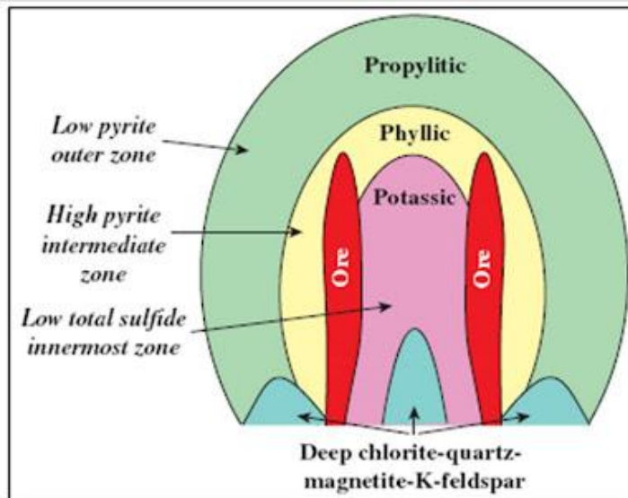
Figure 3.5: Porphyry system alteration zones
