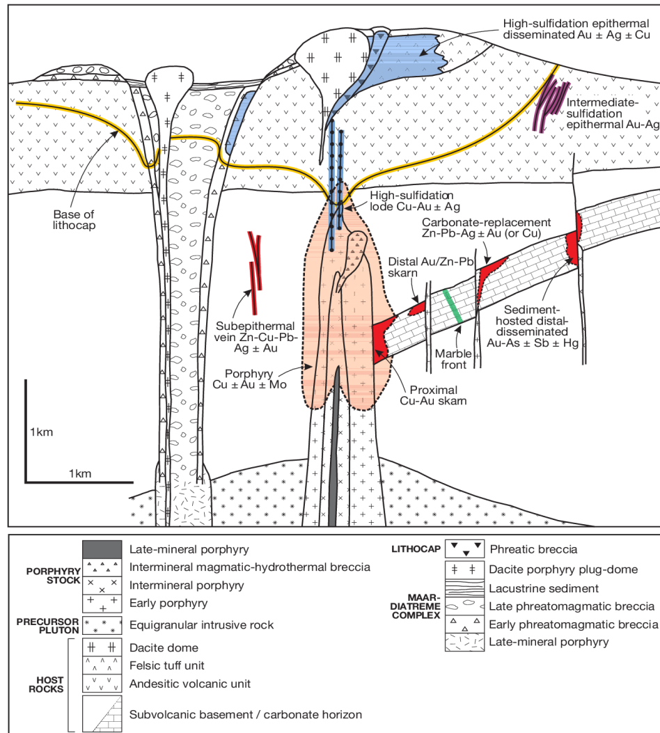
Figure 3.6: Anatomy of porphyry copper system with associated deposit sub-types
