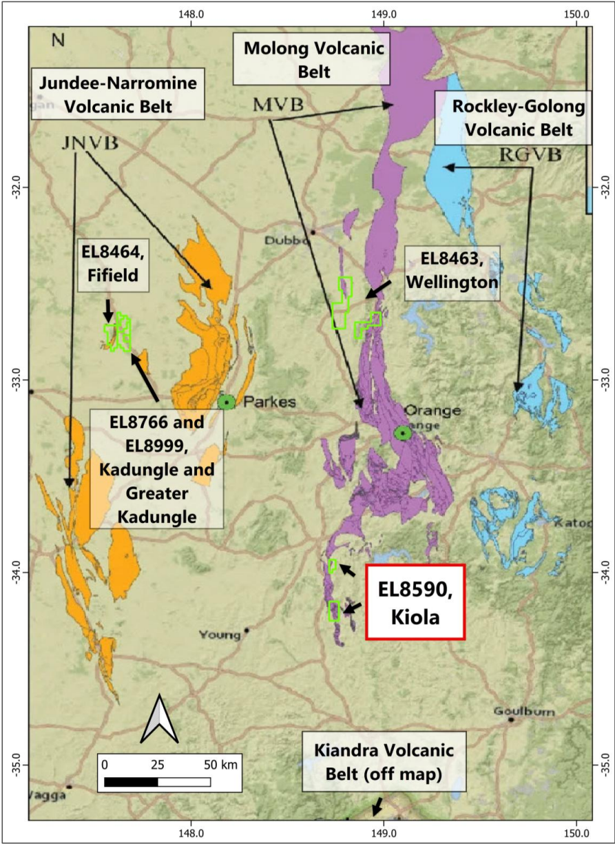
Figure 3.4: Emmerson’s exploration projects – regional geology
