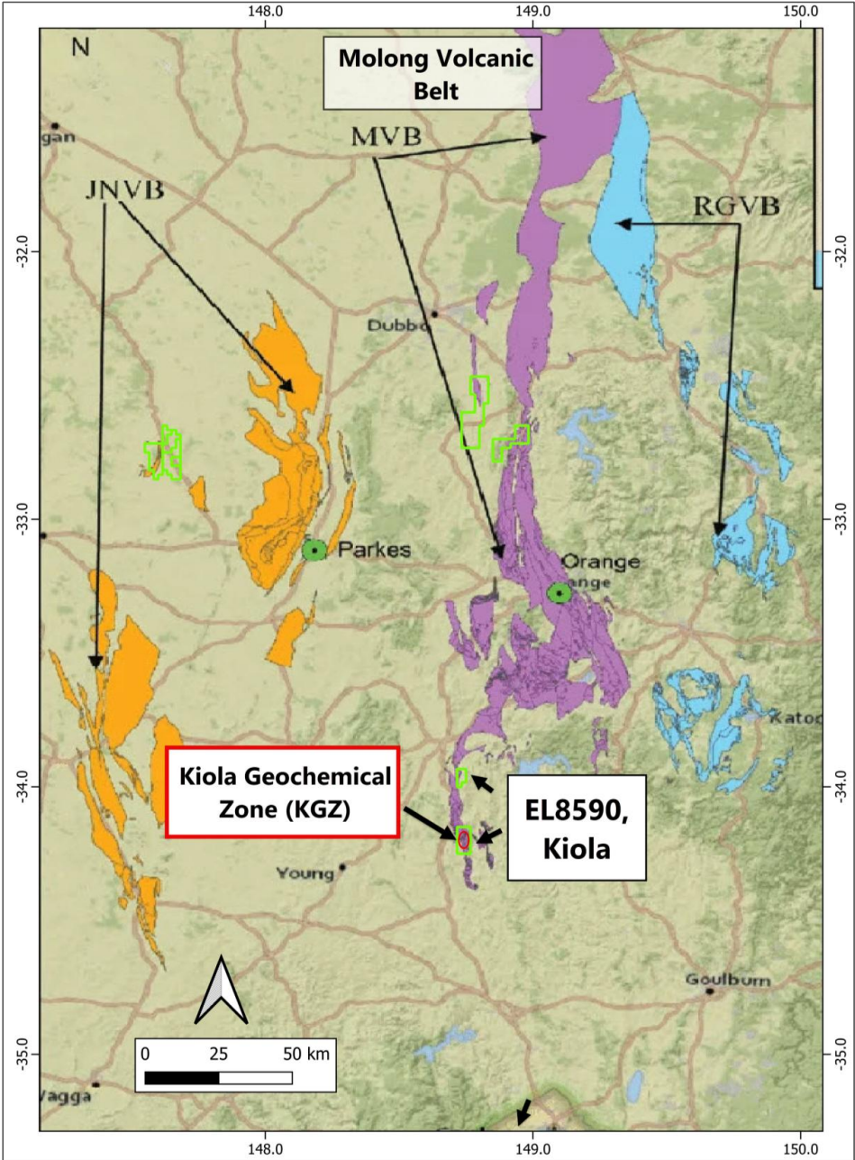
Figure 3.7: Location of Kiola Geochemical Zone on regional map
