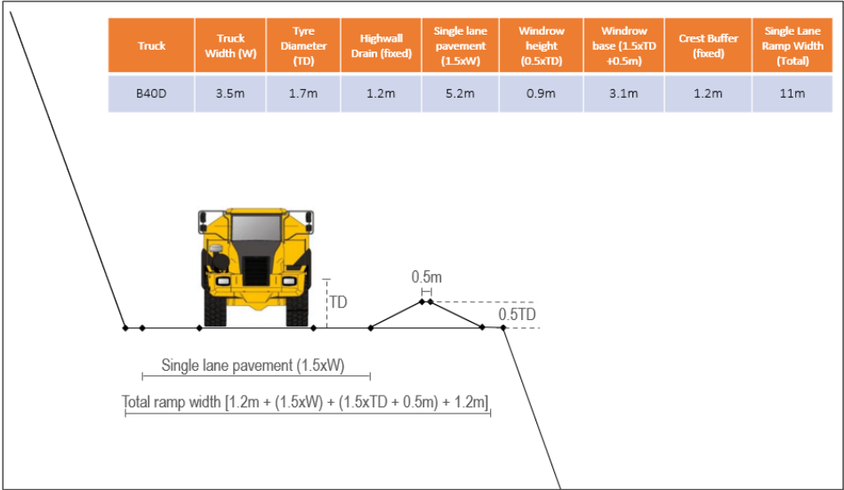
Figure 2.10: Single lane – road width criteria
