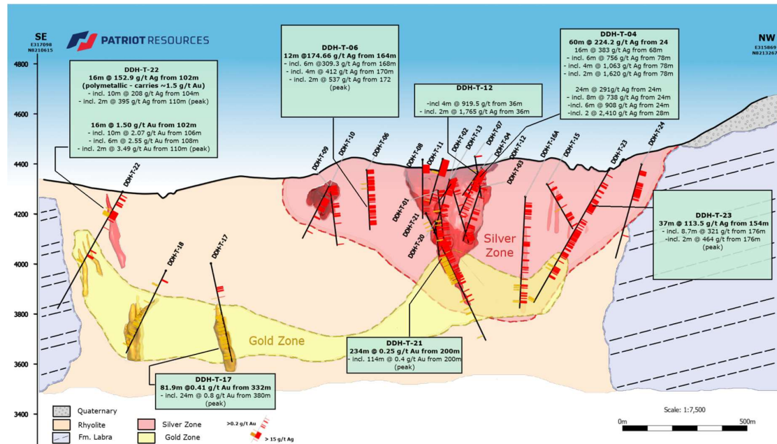
Figure 1: Tassa Cross section showing High Grade Silver and Gold Zones
