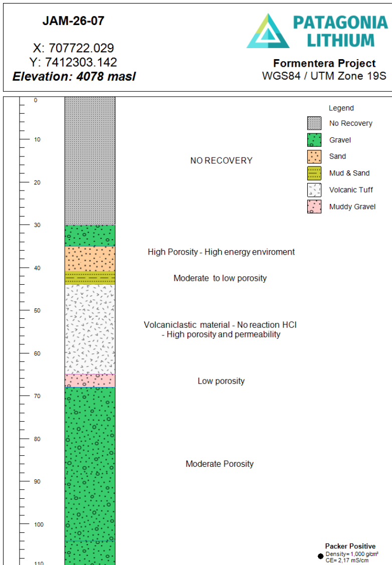
Figure 3. Lithological column from well seven to 110m depth.
