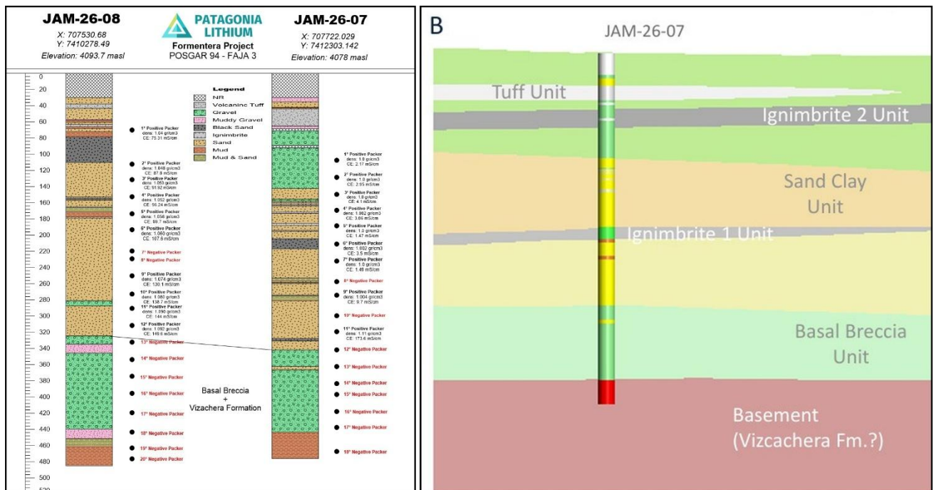
Figure 6. Consistent geology between well 7 and 8 with the sandy aquifer unit tagged by the ignimbrite unit.
