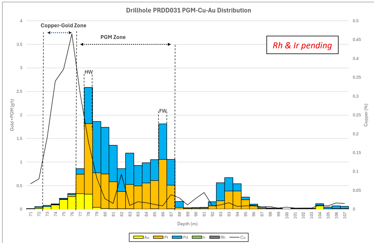
Figure 19: Mineral Distribution Profile for Metallurgical Hole PRDD031
