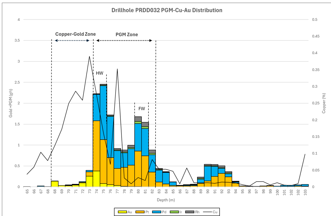
Figure 20: Mineral Distribution Profile for Metallurgical Hole PRDD032
