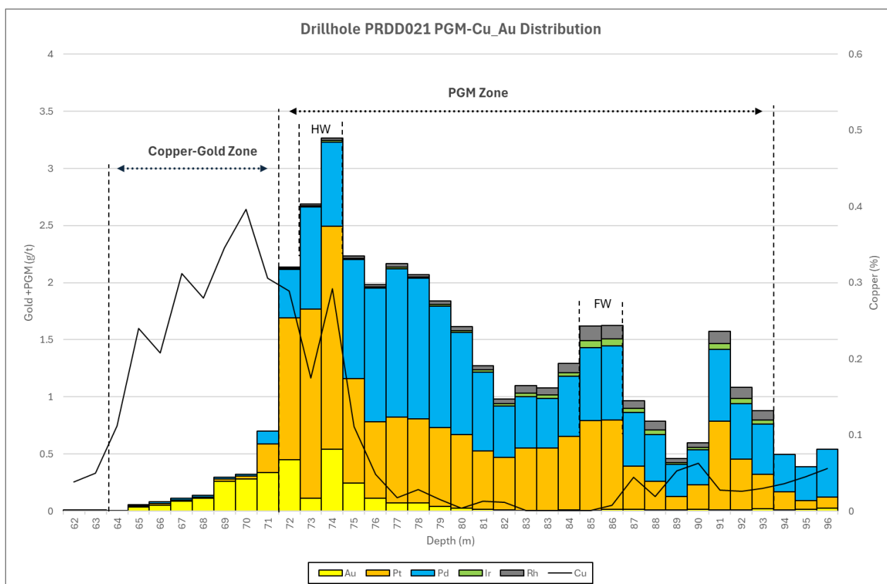
Figure 14: Mineral Distribution Profile for Metallurgical Hole PRDD021
