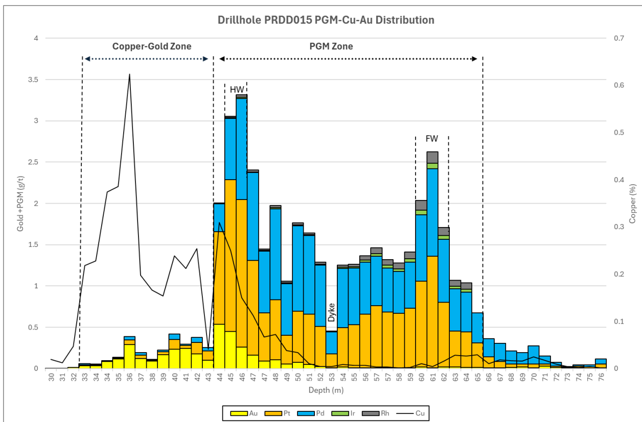
Figure 8: Mineral Distribution Profile for Metallurgical Hole PRDD015
