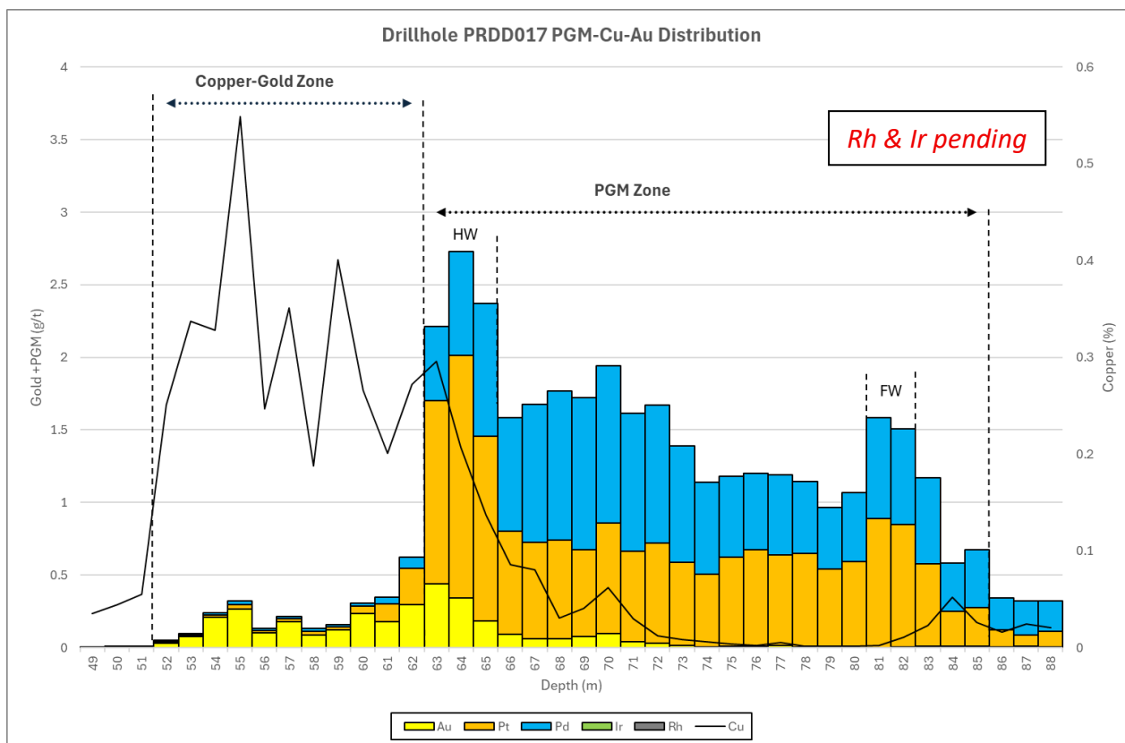
Figure 10: Mineral Distribution Profile for Metallurgical Hole PRDD017
