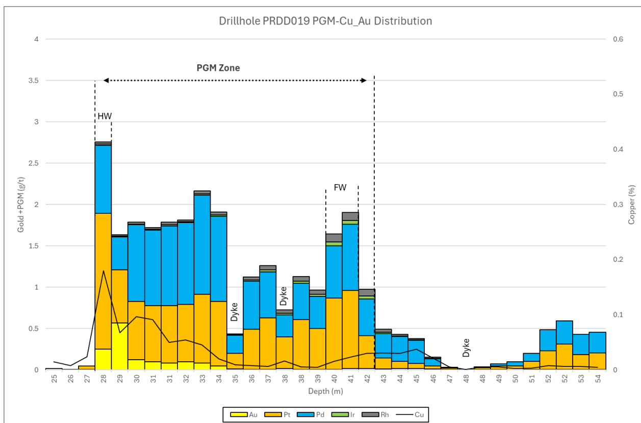
Figure 12: Mineral Distribution Profile for Metallurgical Hole PRDD019
