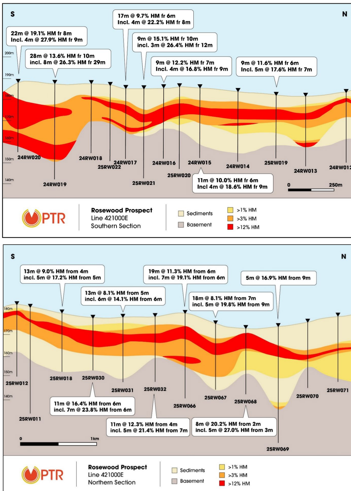
Figure 3: Rosewood Prospect Geological Section Line 421000E. Southern Zone (top) and Northern Zone (below).
