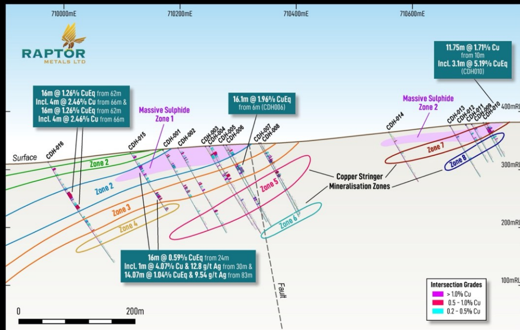
Cross section of Raptor HQ diamond drilling program and interpreted copper stringer and base metal mineralisation zones incorporating drilling completed to date.
