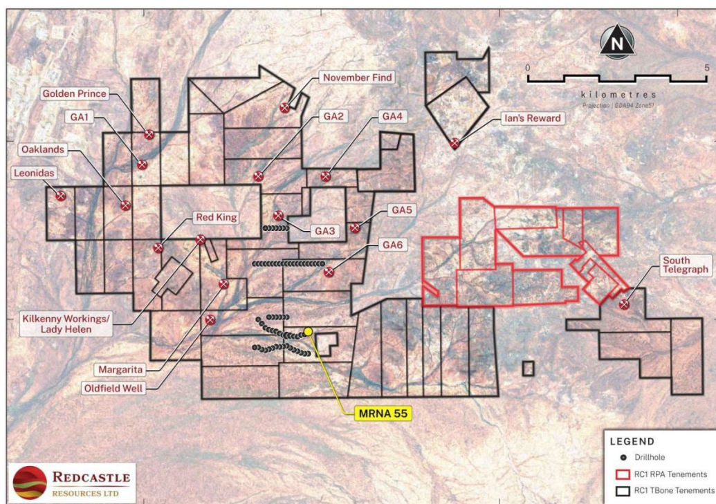
Figure 6. Location of historical drilling completed by Mt Kersey and drillhole MRNA55 (WAMEX Report A52841).
