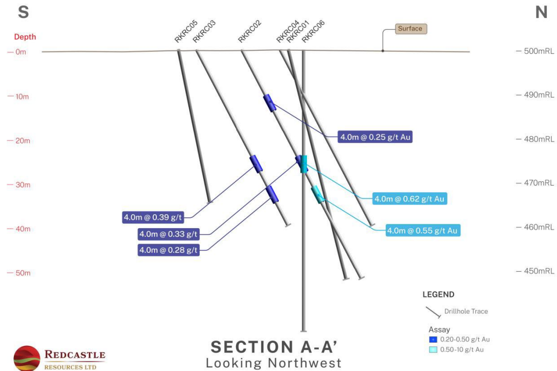
Figure 9. Cross-section showing historical drilling results completed by Connor (WAMEX Report A133775)
