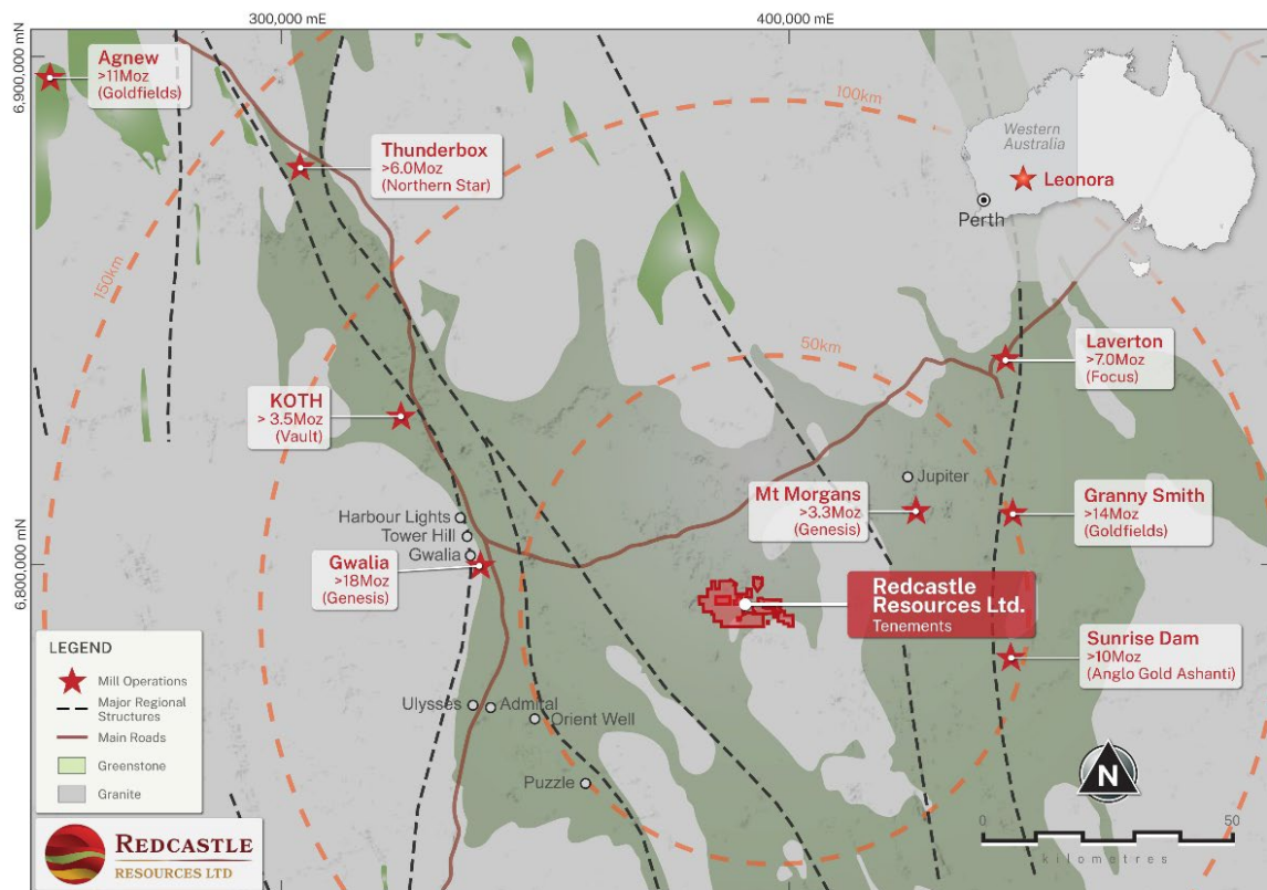
Figure 21. Redcastle Tenements located in the Leonora – Laverton Greenstone Belt
