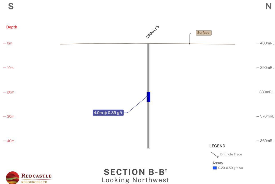
Figure 7. Cross-section showing historical drilling results completed by Mt Kersey (WAMEX Report A52841).
