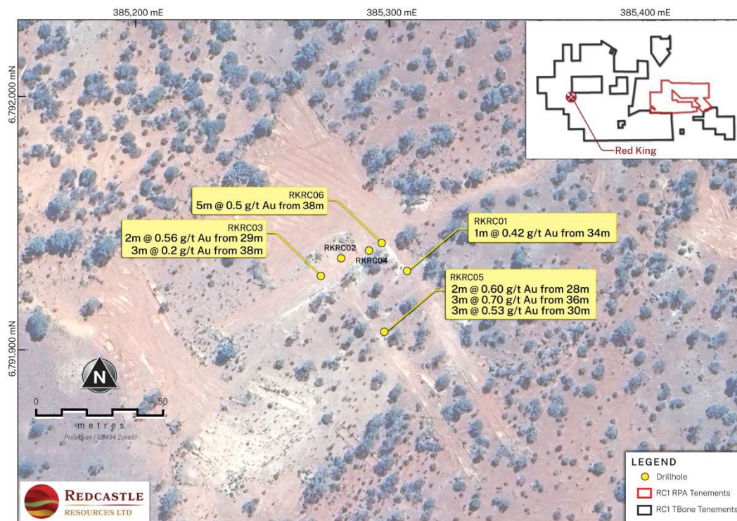
Figure 8. Historical drilling location as carried out by Connor (WAMEX Report A133775)
