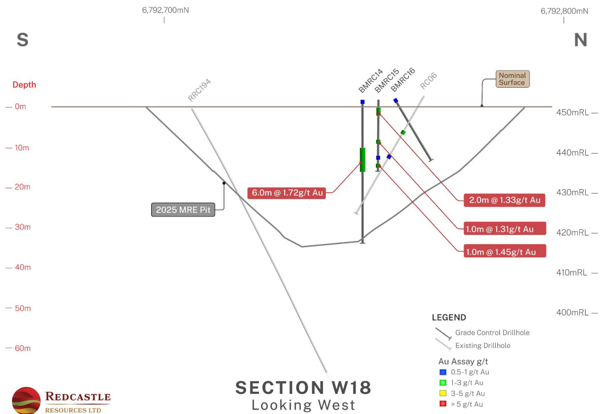
Figure 10 Section W18 showing recent GC drilling (Uncut Gold Values)
