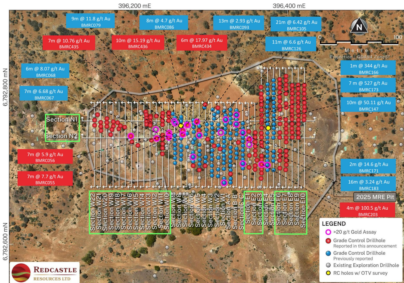
Figure 1 Plan view of GC drillhole locations and significant gold assays. Sections reported in this announcement are highlighted in green. Gold values are uncut.
