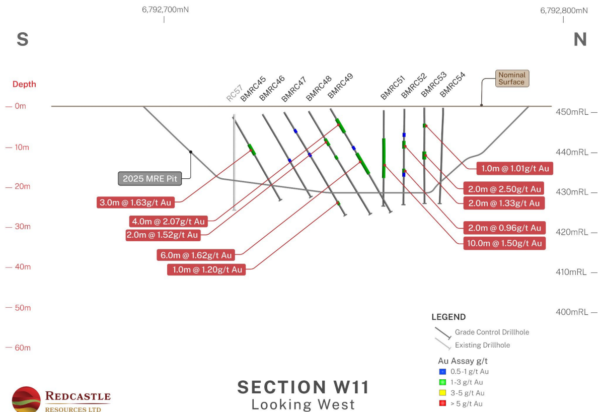
Figure 3 Section W11 showing recent GC drilling (Uncut Gold Values)
