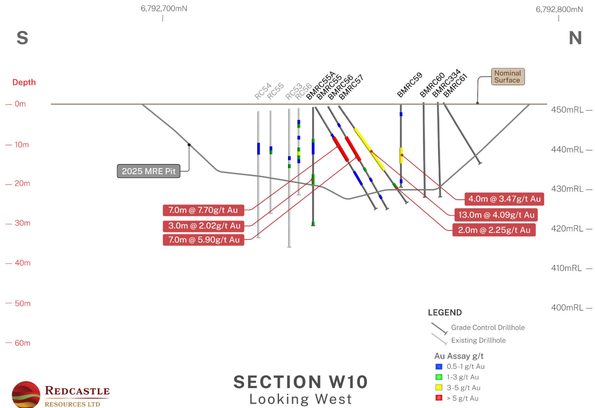
Figure 2 Section W10 showing recent GC drilling (Uncut Gold Values)
