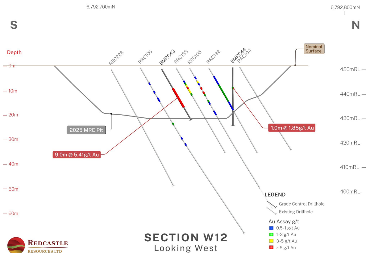
Figure 4 Section W12 showing recent GC drilling (Uncut Gold Values)
