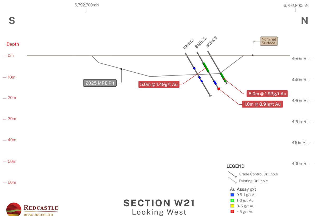
Figure 13 Section W21 showing recent GC drilling (Uncut Gold Values)
