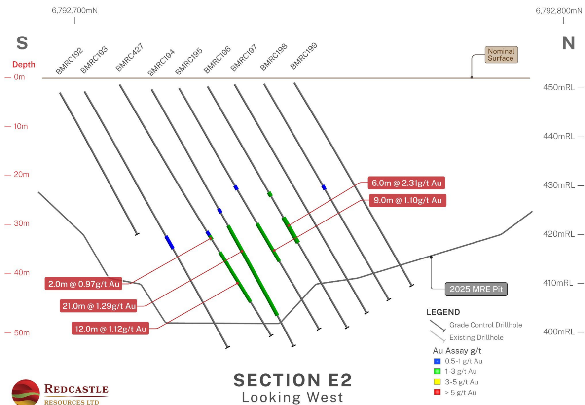
Figure 16 Section E2 showing recent GC drilling (Uncut Gold Values)
