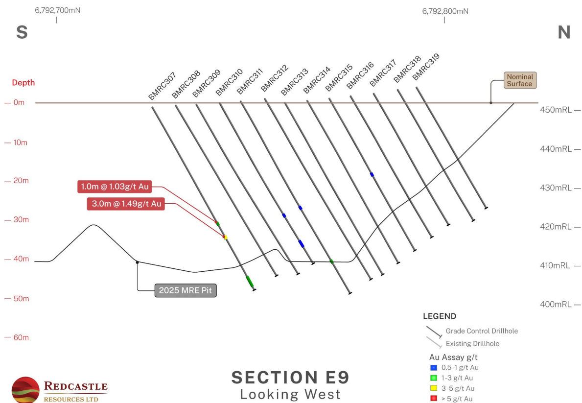
Figure 21 Section E9 showing recent GC drilling (Uncut Gold Values)
