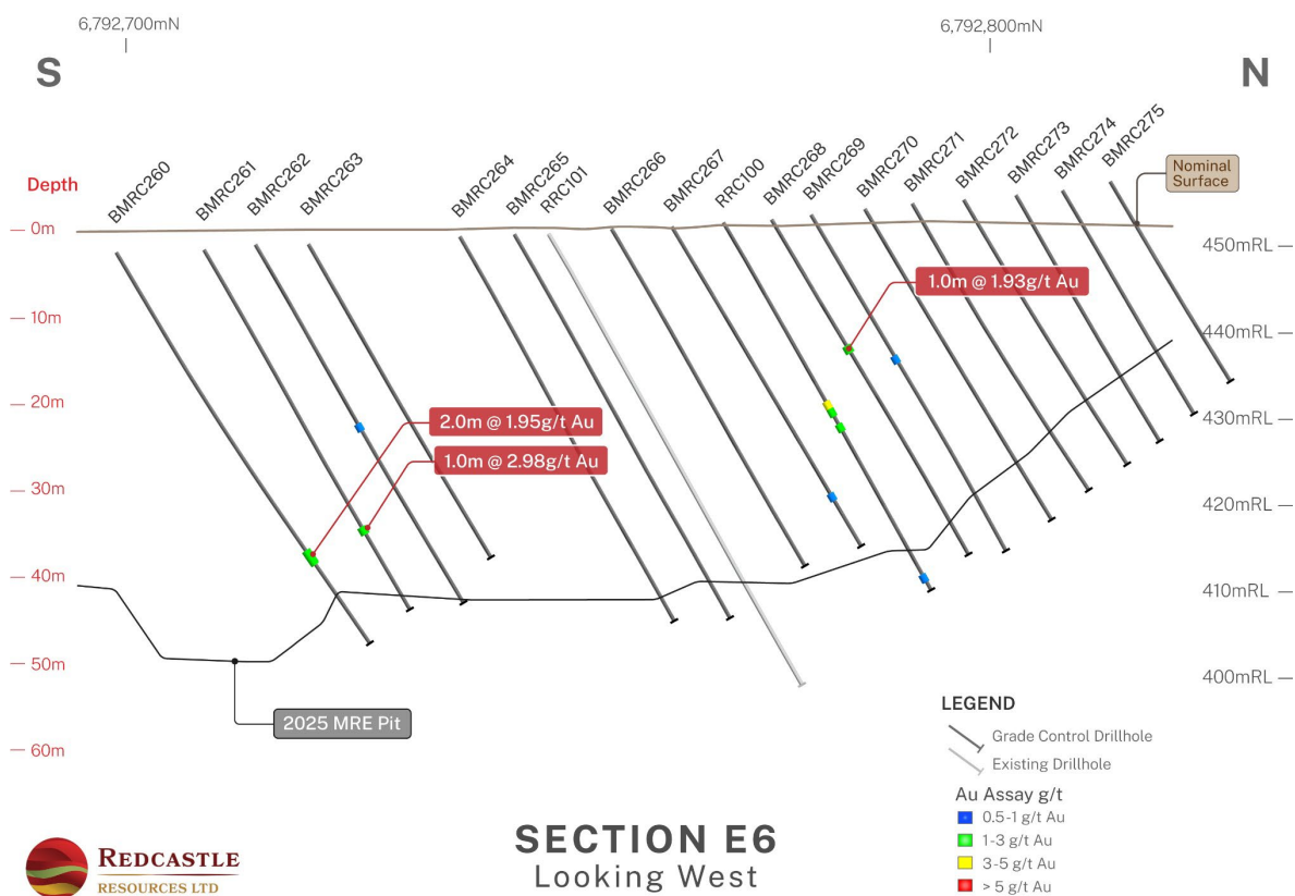
Figure 18 Section E6 showing recent GC drilling (Uncut Gold Values)
