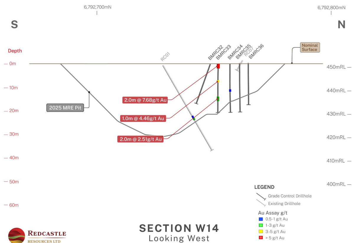
Figure 6 Section W14 showing recent GC drilling (Uncut Gold Values)
