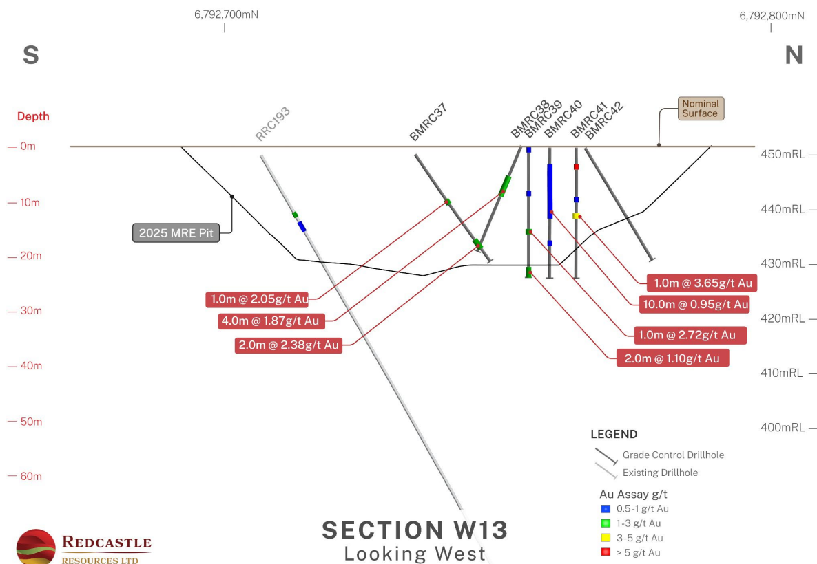
Figure 5 Section W13 showing recent GC drilling (Uncut Gold Values)
