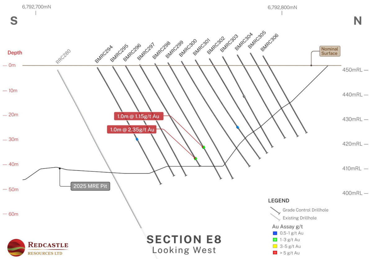
Figure 20 Section E8 showing recent GC drilling (Uncut Gold Values)
