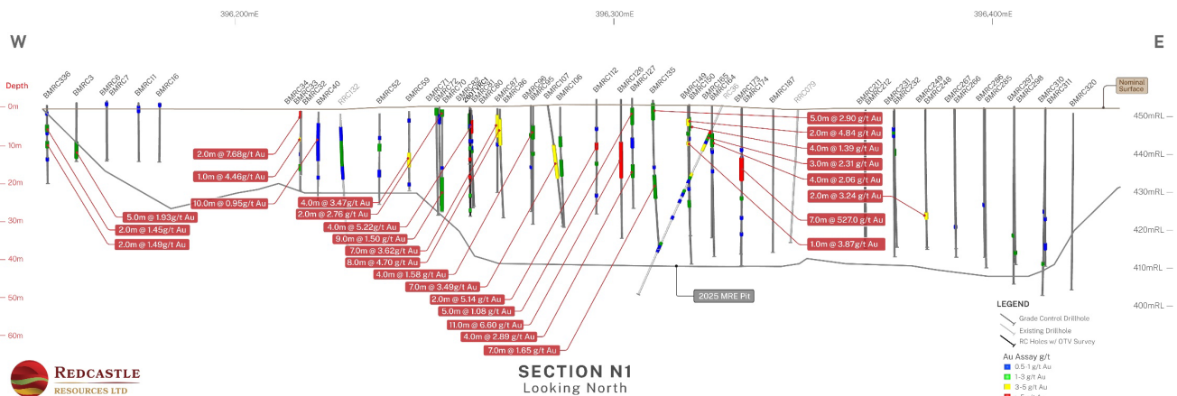
Figure 23 Long Section N1 showing recent GC drilling (Uncut Gold Values) with mineralised trend towards the east
