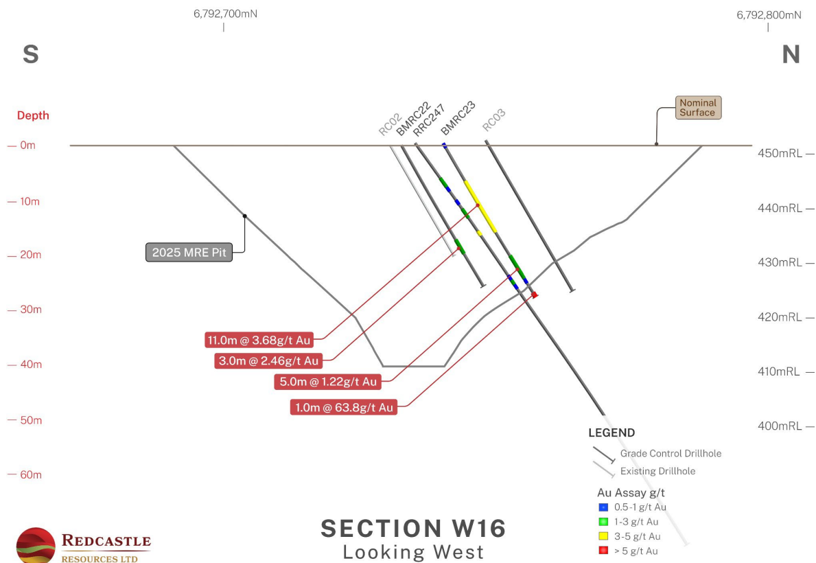
Figure 8 Section W16 showing recent GC drilling (Uncut Gold Values)
