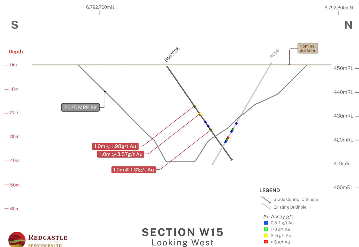
Figure 7 Section W15 showing recent GC drilling (Uncut Gold Values)
