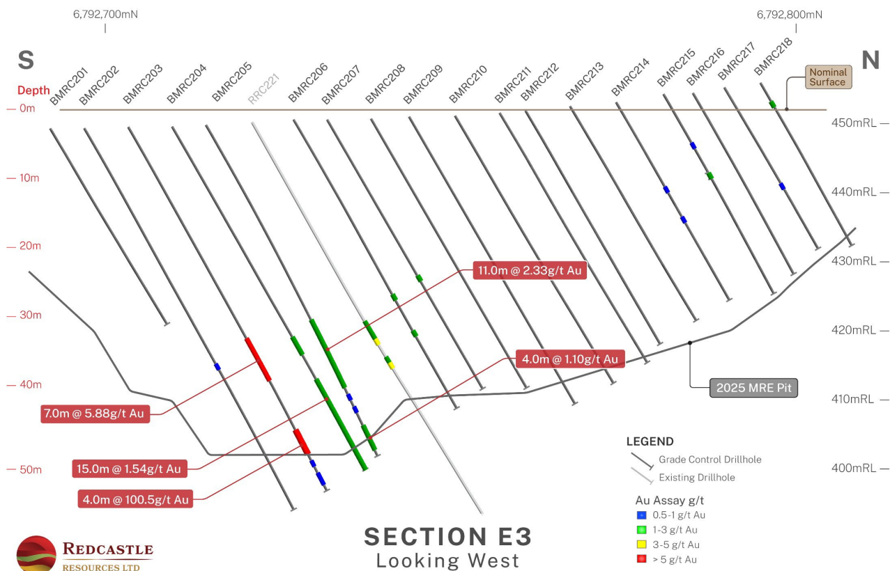
Figure 17 Section E3 showing recent GC drilling (Uncut Gold Values)
