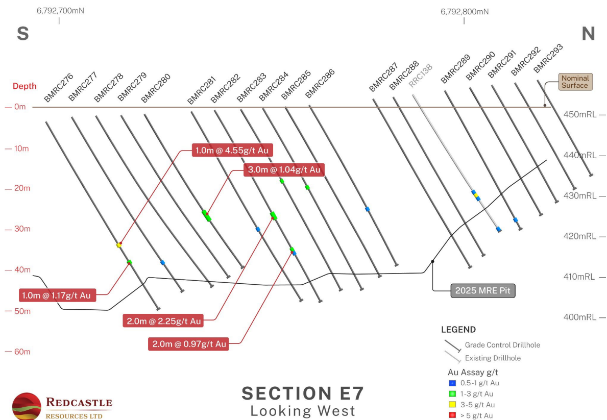
Figure 19 Section E7 showing recent GC drilling (Uncut Gold Values)
