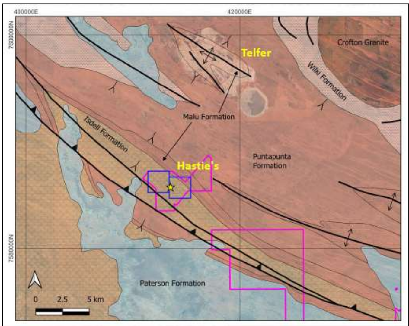
Figure 2 - South Telfer Area Regional Geology
