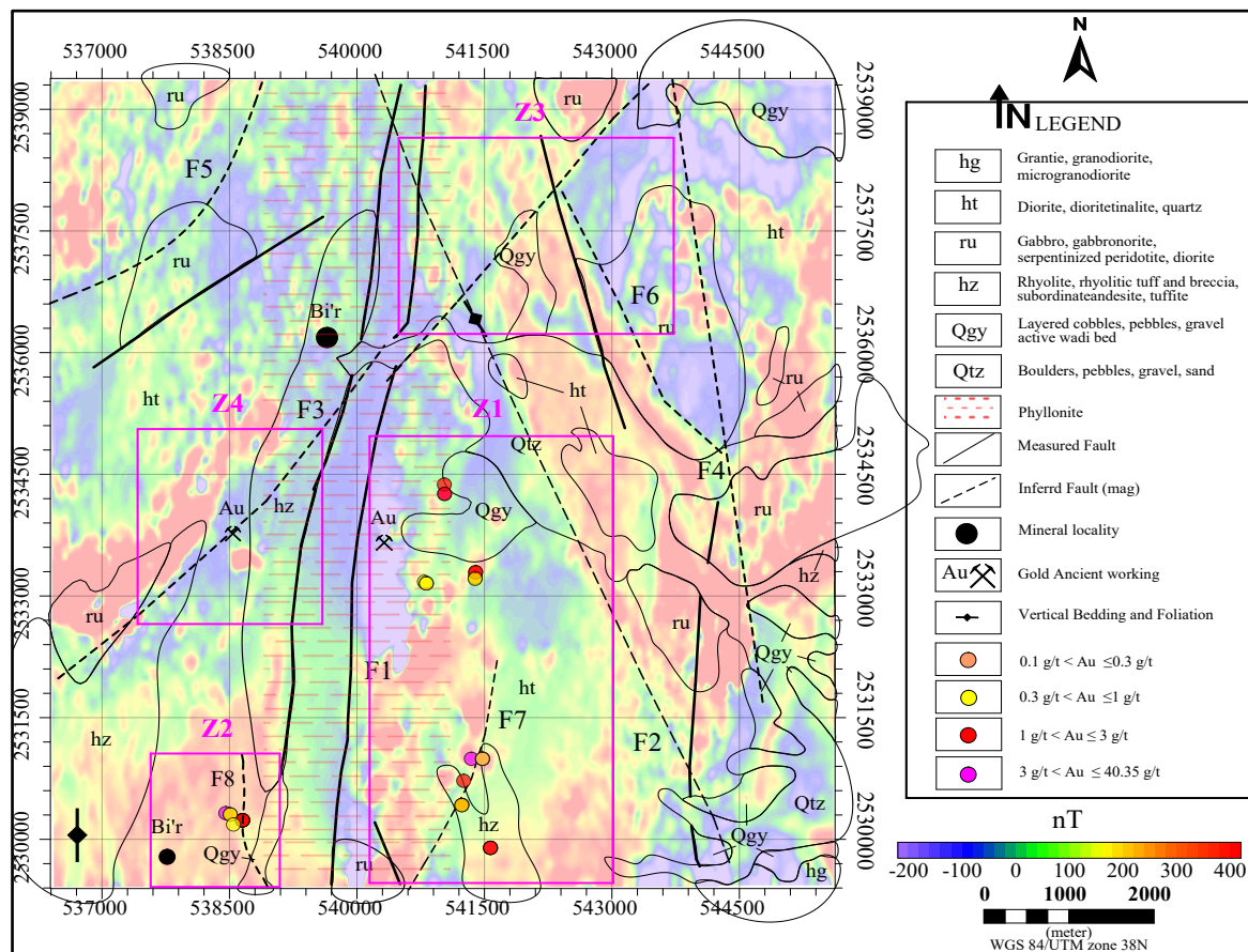
Figure 6. Target Zones (Z1-Z4), Rock Samples on RTP Magnetic Anomaly Map, Shaib Marqan Area (on TMI IVD; EPSG 32638: WGS84 UTM 38N)
