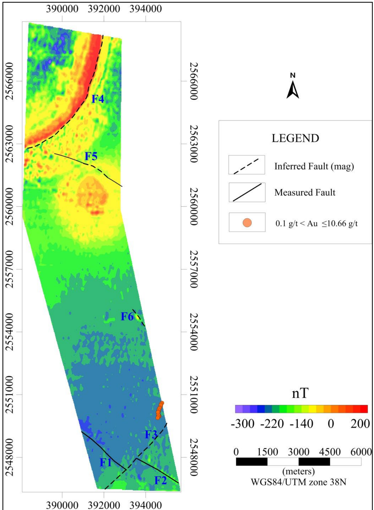
Figure 3. RTP Magnetic Anomalies and Inferred Structures of the Wadi Salamah Area
