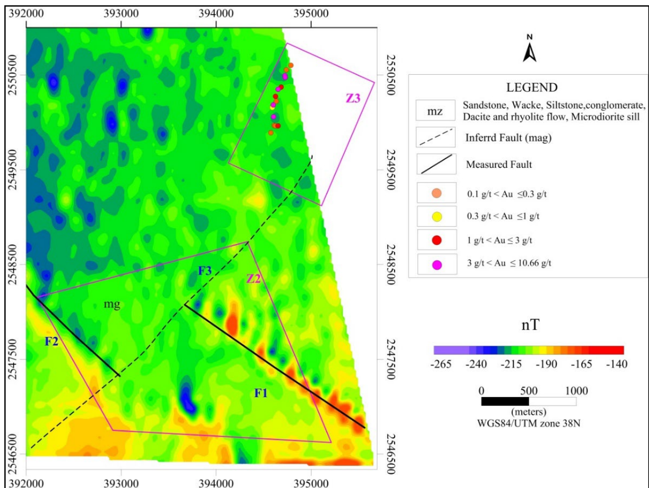
Figure 5. Geological Map, Magnetic Anomalies and their inferences of the Z2 and Z3 Area on TMI (EPSG 32638: WGS84 UTM 38N)
