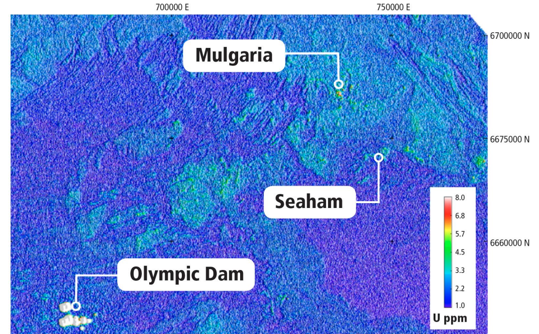
Comparison of the Mulgaria anomalous radiometric response to nearby Seaham uranium prospect (image approximately 1,600km 2 ).*
