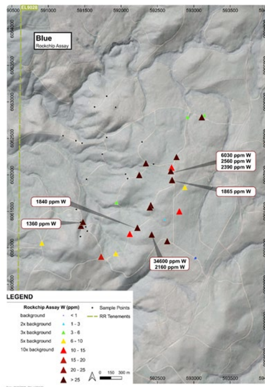
Figure 3: Tungsten (W) high-grade certified rock chip results occur within the defined anomaly.
