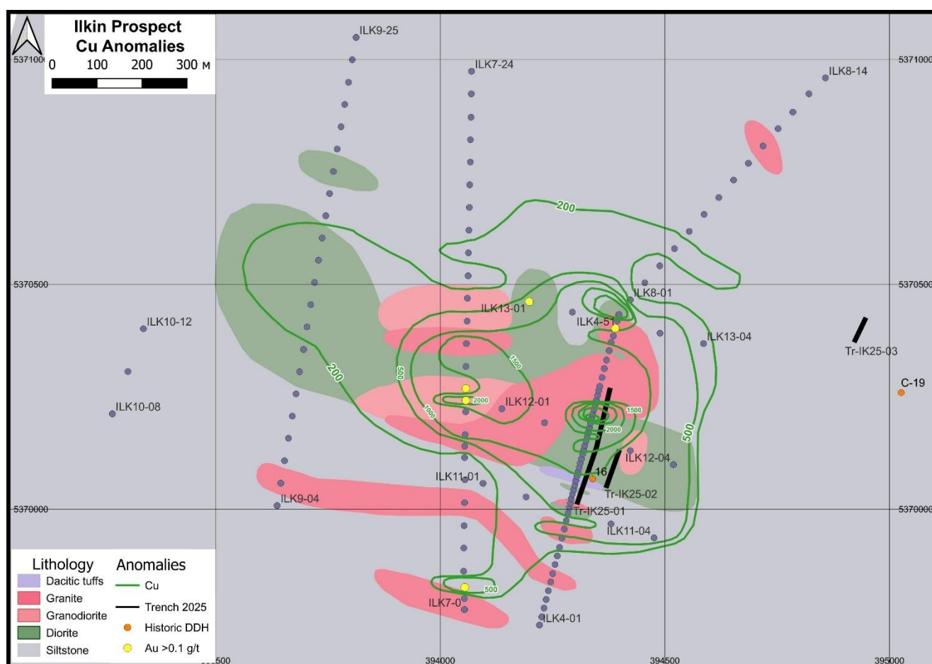
Figure 1 – Lithology map with copper and gold anomalism of the Ilkin Prospect at Baynazar.
