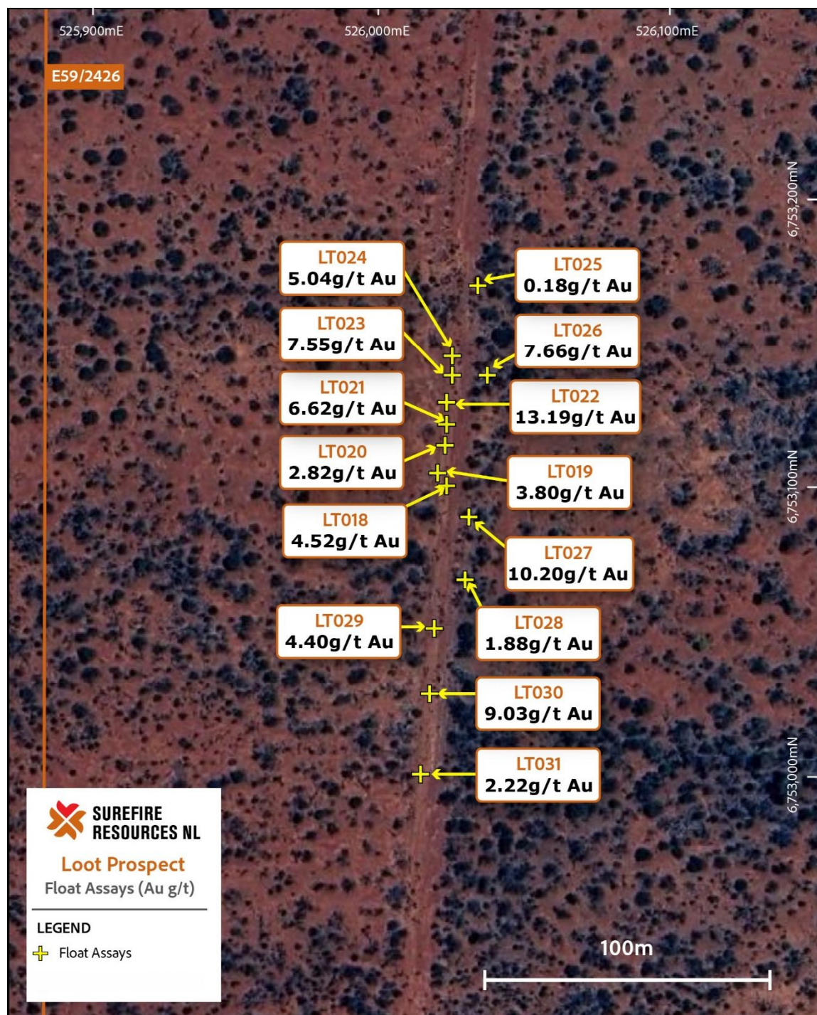
Figure 1 Plan showing float rock sampling of Albitite lithology
