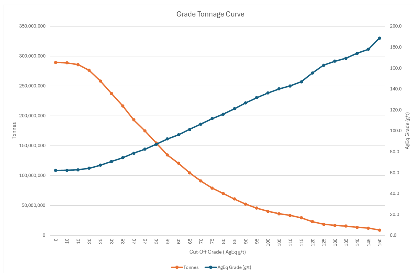
Figure 5 - Grade Tonnage Curve of Maverick Springs 2025 Mineral Resource Upgrade <150g/t AgEq cutoff (ID 2 Estimate)
