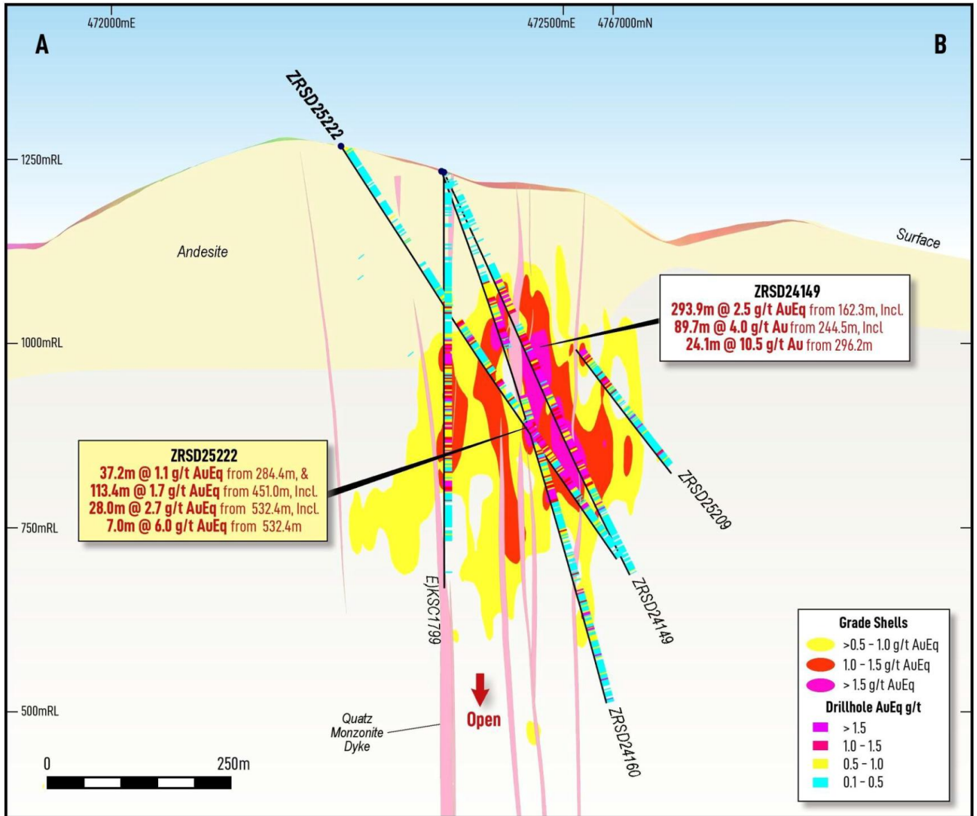
Figure 3: Shanac cross-section view looking NW (25m view width), showing drill-hole traces with intercepts, geology and AuEq grade shells.
