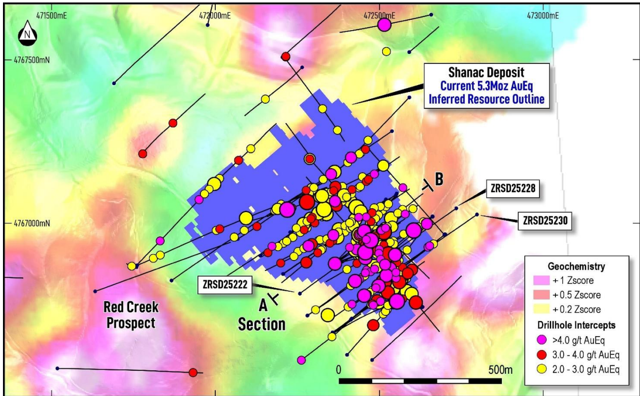
Figure 2: Plan view map of the Shanac deposit, showing resource footprint, drill-hole collars and traces, high-grade intercept points and background Au-Ag in soil geochemistry.
