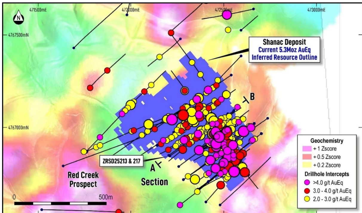
Figure 7. Plan view map of the Shanac deposit, showing the resource footprint, drill-hole collars and traces, high-grade intercept points and background Au-As in soil geochemistry.
