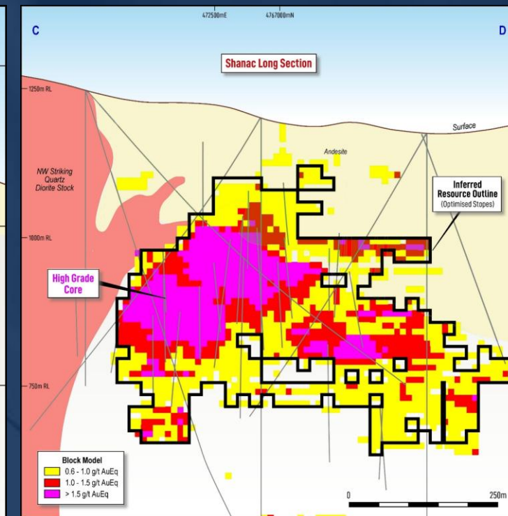
Shanac long section view, looking west
