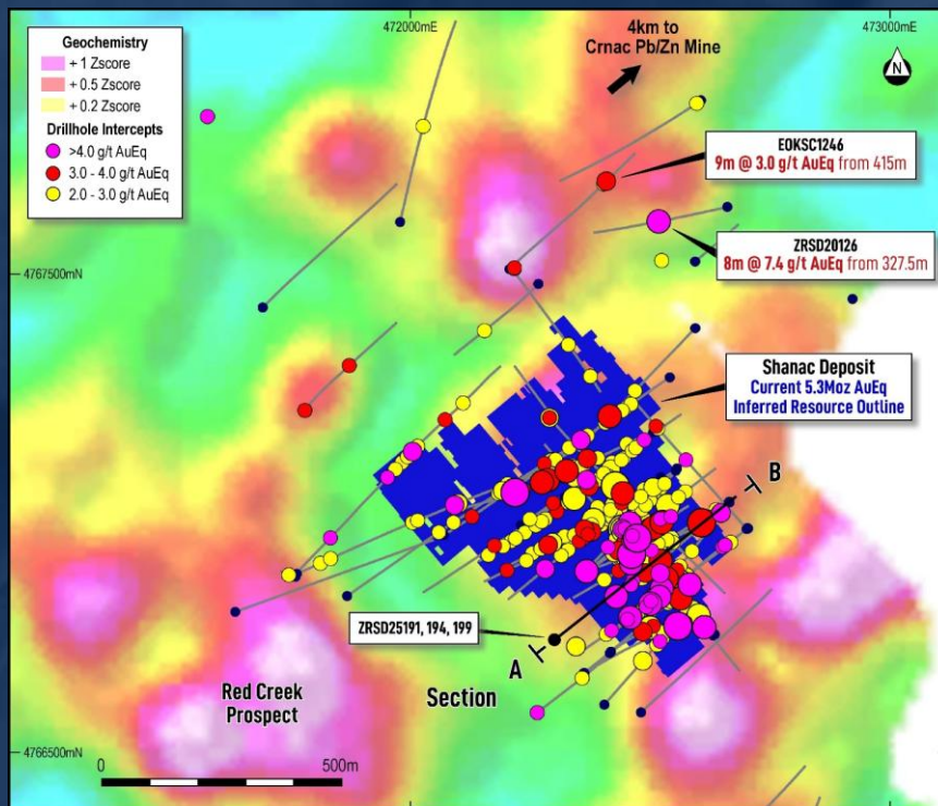
Shanac plan view map
