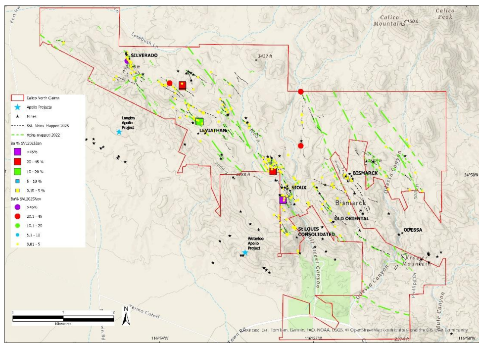
Figure 5. Calico North project, barite assay results. Note samples from Leviathan Barite Mine returned results of 10-20%, while other targets show results of greater than 20% Barite.
