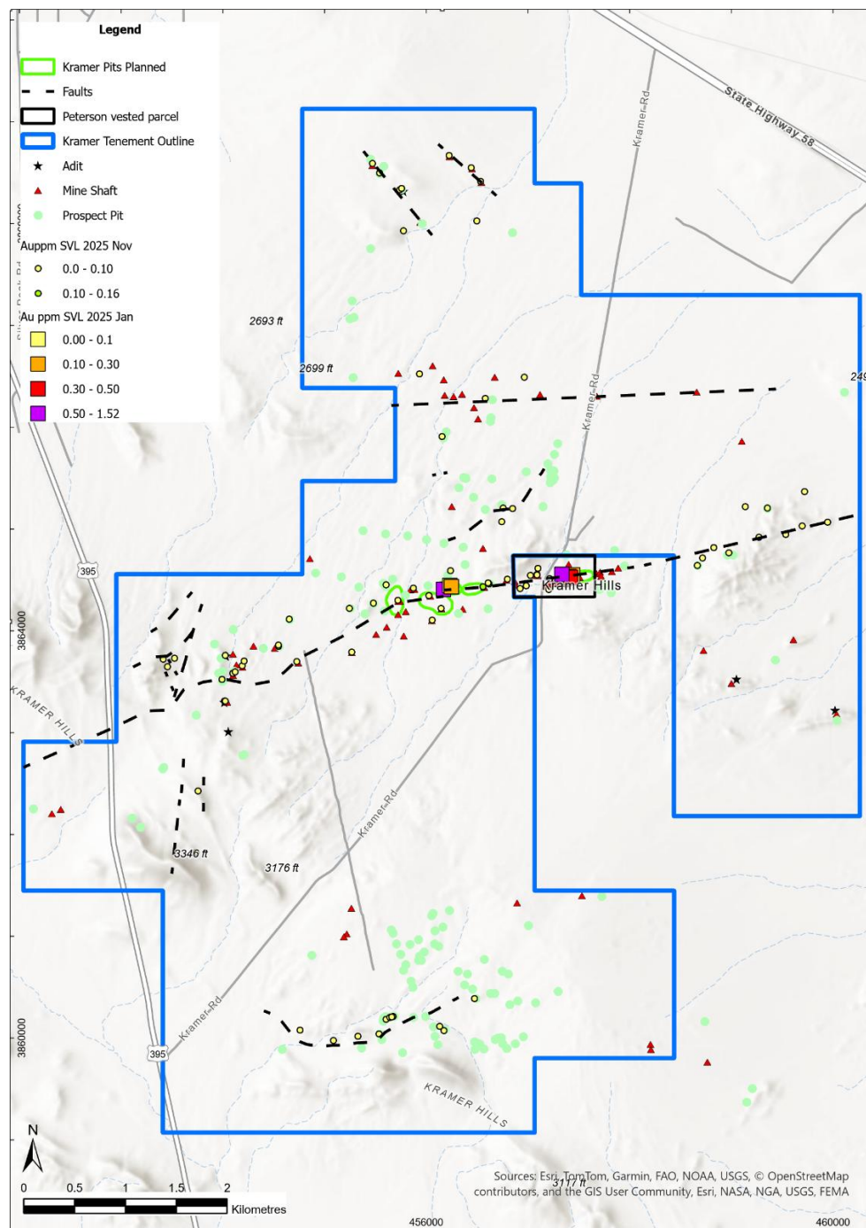
Figure 6. Kramer Hills Claim Map with Historic Workings and Faults. Note the exploration potential for areas outside of pits permitted for mining in the 1980's. A mapped and inferred fault running through the prospect area extends for over 7 km, aligned with pre-1942 mine shafts. There are also various repeated faults and lines of historical shafts that are prospective.
