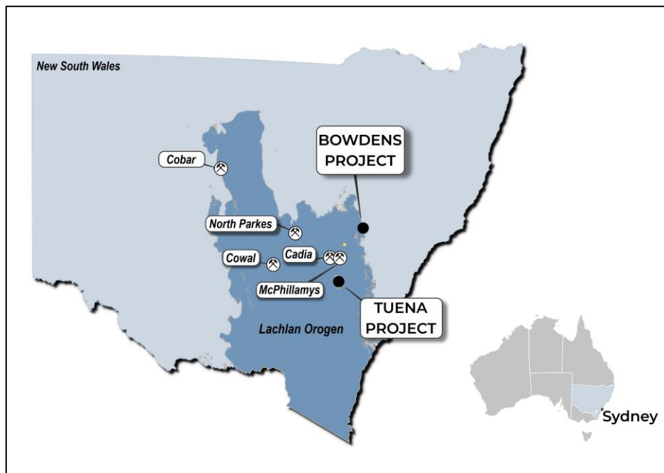
Figure 9. Silver Mines Limited project in the Lachlan Orogen.
