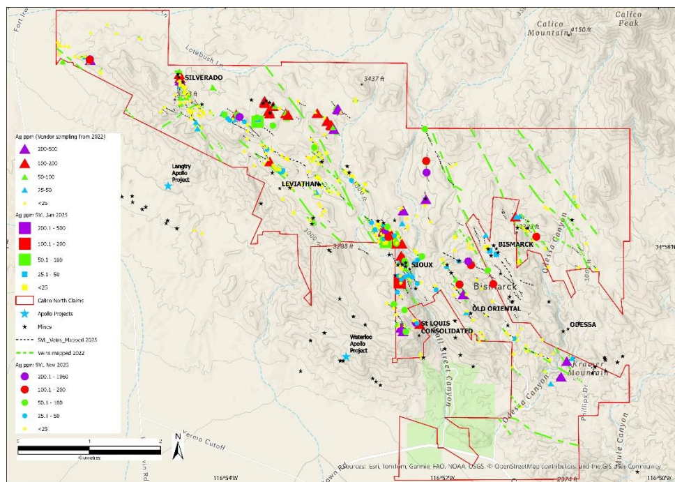
Figure 4. Calico North project, silver assay results, showing mapped veins and results of rock chip sampling. Note the number of clusters with good silver grades that will be followed up by drilling. It is possible that these clusters, are controlled by intersecting vein systems and stratigraphy.
