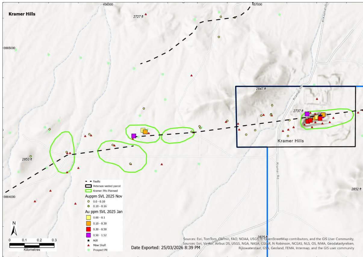
Figure 7. Zoomed view of the oxide prospect area. Note alignment with a mapped fault zone and presence of mine shafts that are spread along the zone, which were all worked prior to 1942. Silver Mines verification samples taken in 2025, confirm presence of mineralised system.
