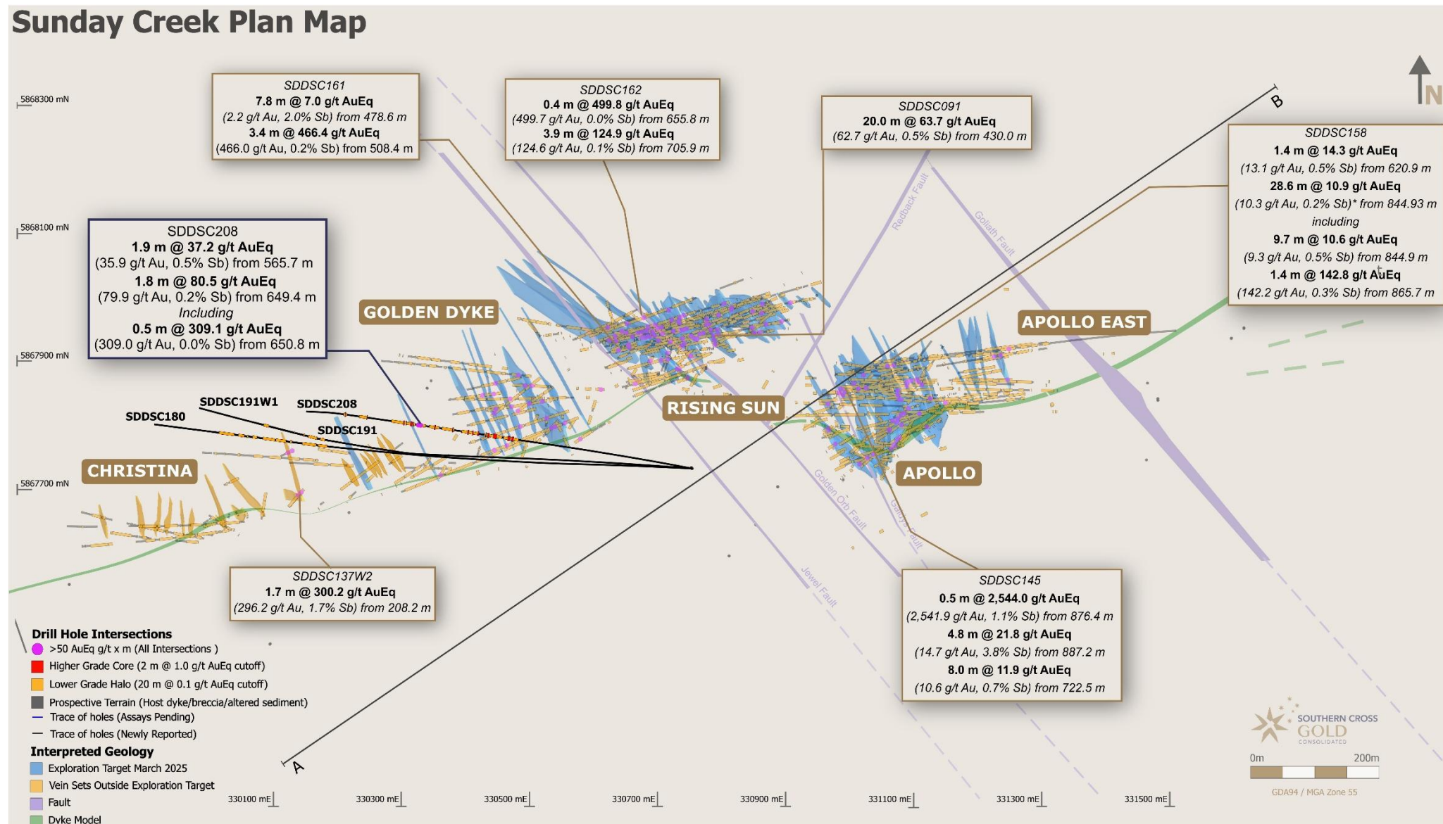
Figure 2: Sunday Creek plan view showing selected results from holes SDDSC180, SDDSC191, SDDSC191W1 and SDDSC208 reported here (dark blue highlighted box, black trace), with selected prior reported drill holes.
