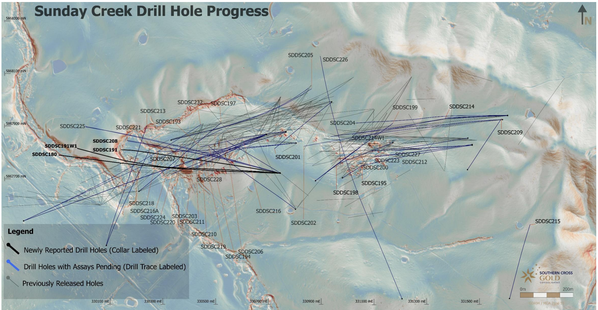
Figure 3: Sunday Creek plan view showing selected drillhole traces from holes SDDSC180, SDDSC191, SDDSC191W1 and SDDSC208 reported here (black trace), with prior reported drill holes (grey trace) and currently drilling and assays pending hole traces (dark blue).
