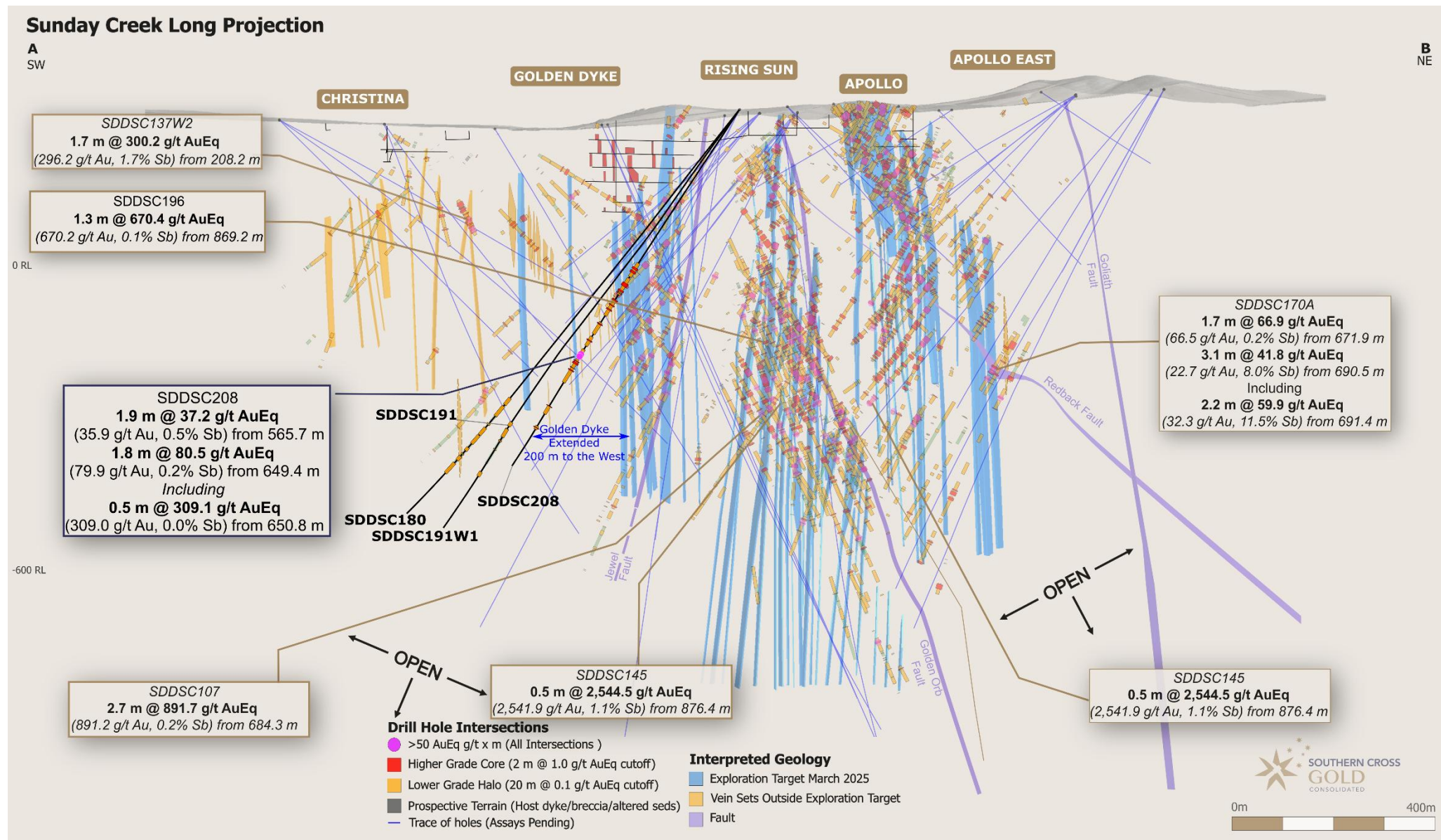
Figure 4: Sunday Creek longitudinal section across A-B in the plane of the dyke breccia/alterated sediment host looking towards the NW (striking 56 degrees) indicating mineralized vein sets. Showing holes SDDSC180, SDDSC191, SDDSC191W1 and SDDSC208 reported here (dark blue highlighted box, black trace), with selected intersections and prior reported drill holes. The vertical extents of the vein sets are limited by proximity to drill hole pierce points.
