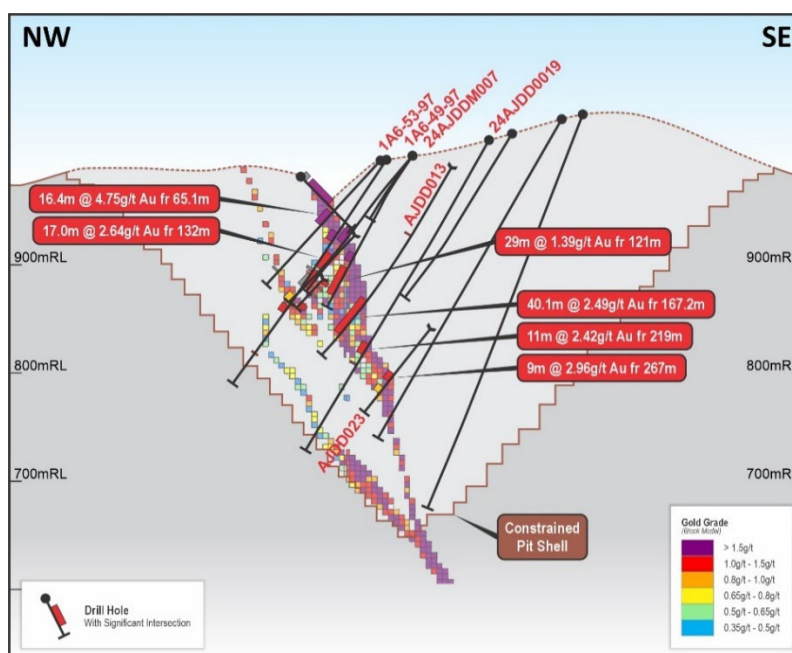
Figure 7-6 | Jonction Block Model - Representative Cross Section
