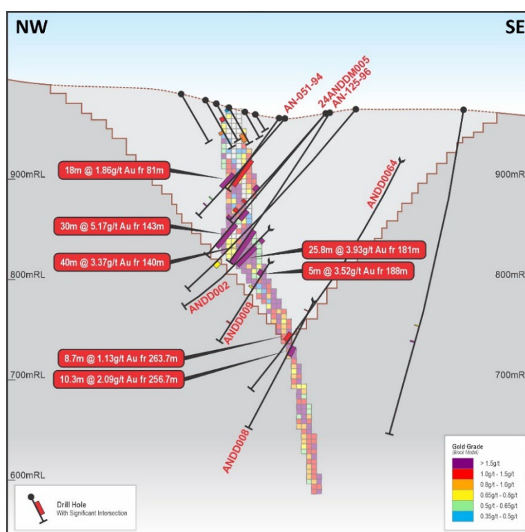
Figure 7-7 | Anuiri Block Model – Representative Cross Section
