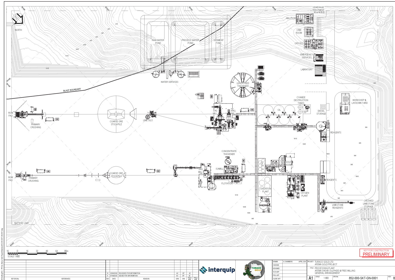
Figure 14-2 | Process Plant Layout
