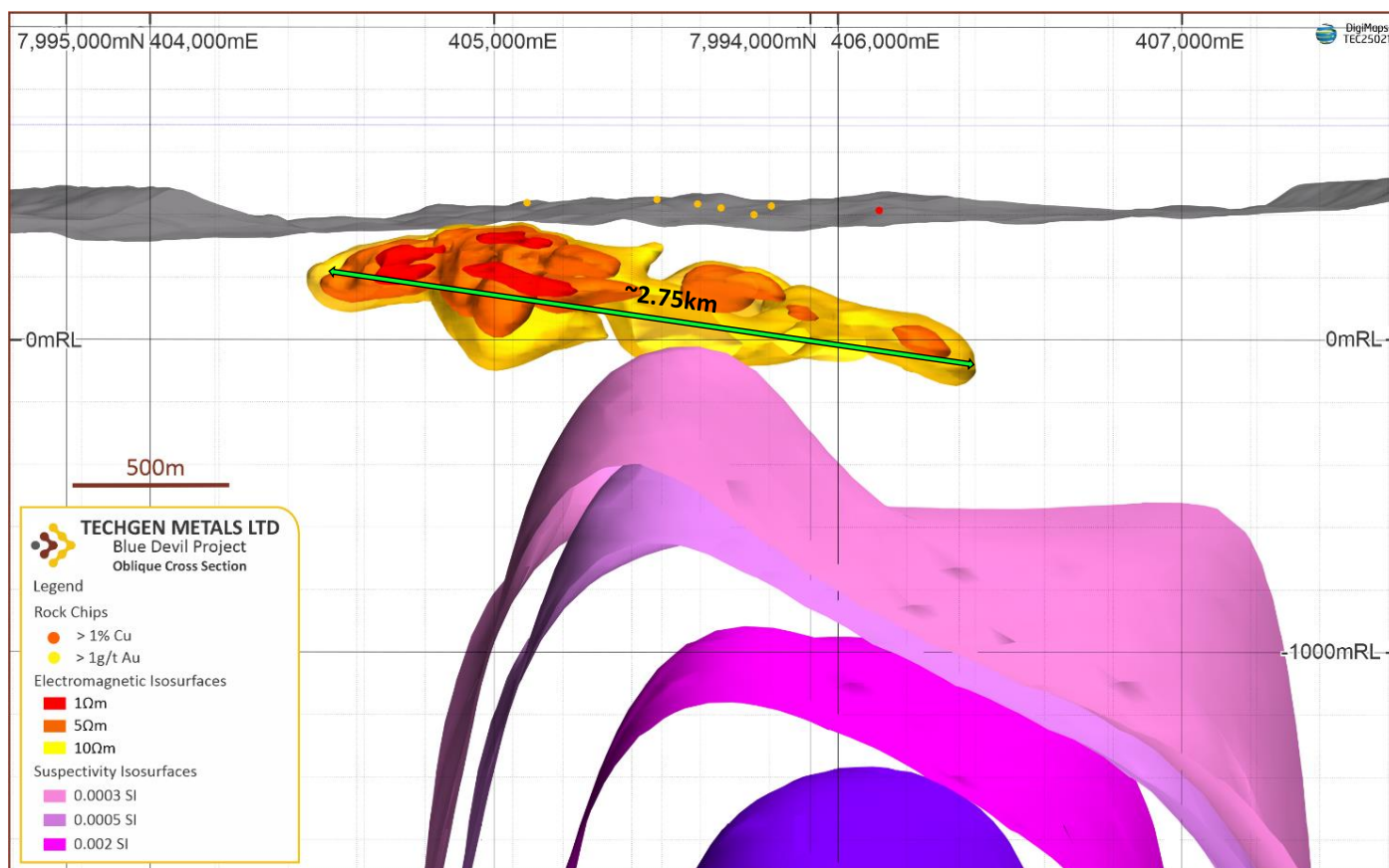
Figure 3: Blue Devil Airborne EM (Yellow/Red) Target with magnetic intrusive (Pink/Purple).
