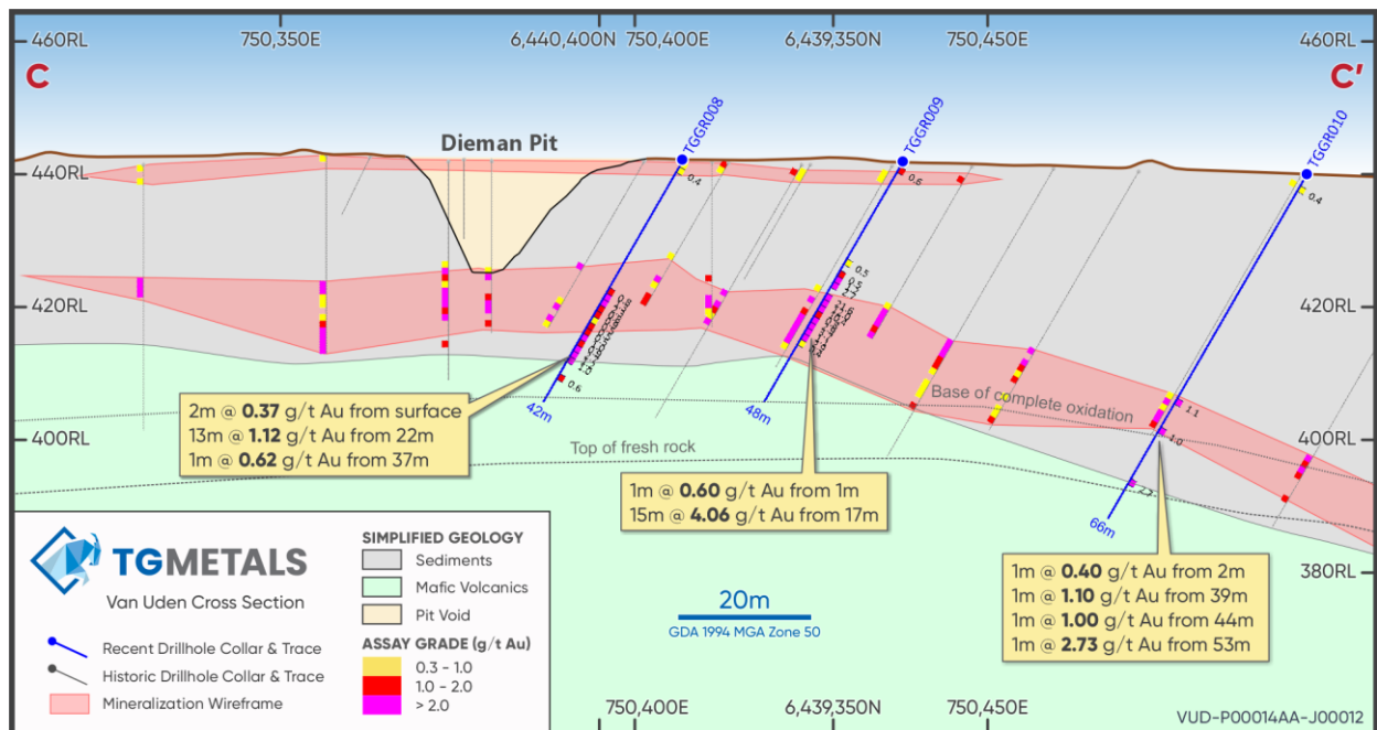
Figure 5 – Cross Section C-C' Showing new drilling, historical drilling and the Van Uden mineralisation envelope
