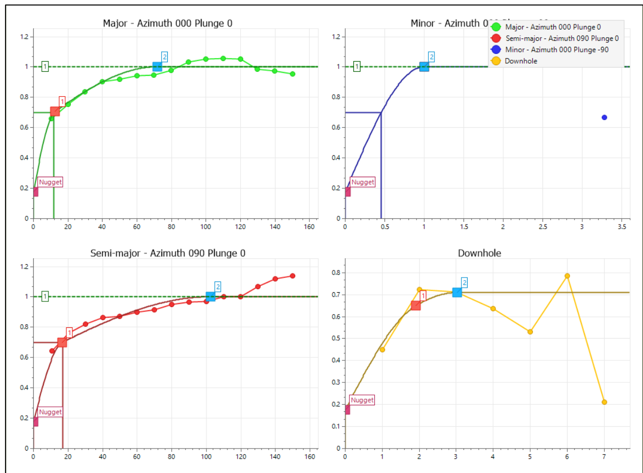
Figure 12 Laterite Variography
