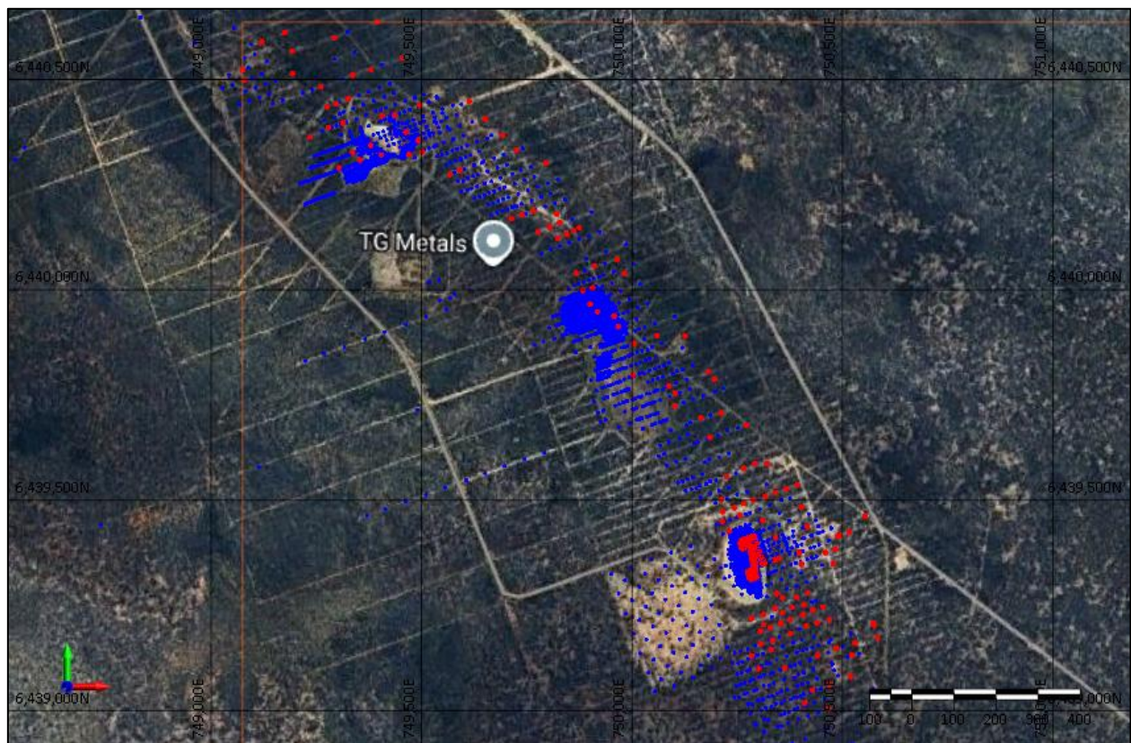
Figure 3 Drill Hole Location Plan
