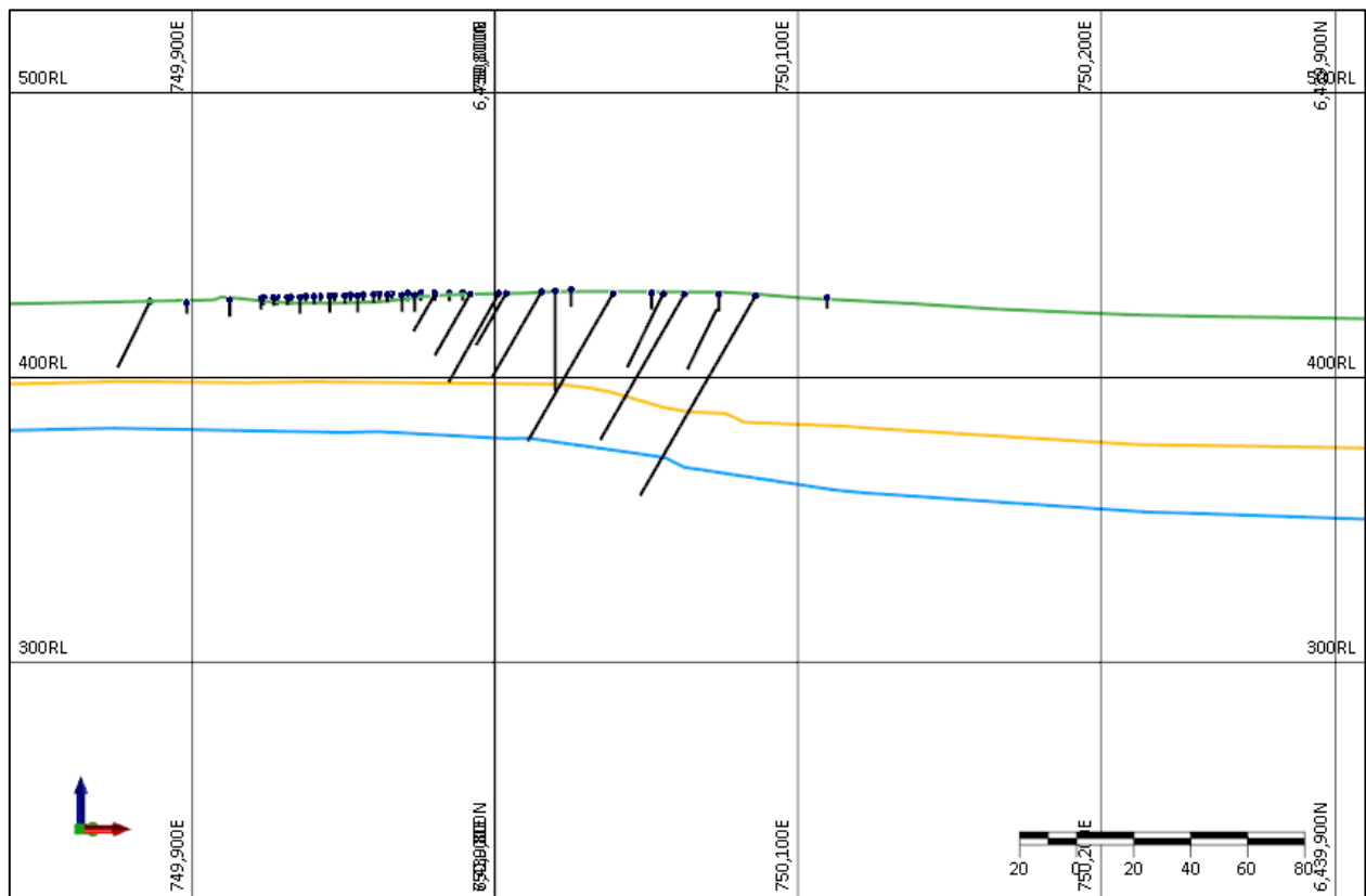
Figure 5 Weathering Surfaces
