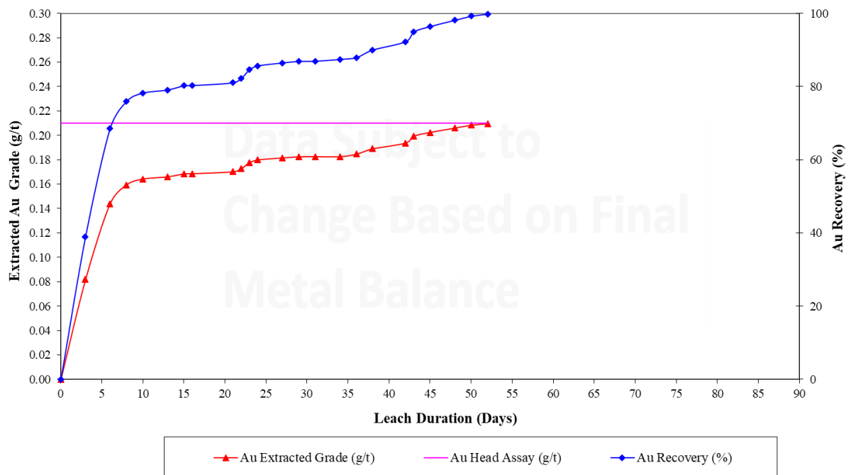
Figure 3 - Leaching Times for Column Two Leach Tests
