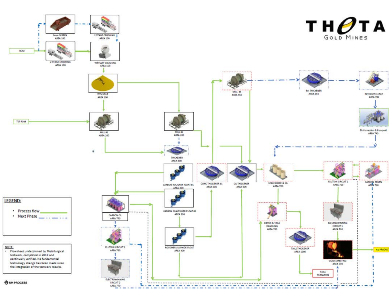
Figure 20: Process Flow Schematic by RM Process Showing both the New and Expanded Plant
