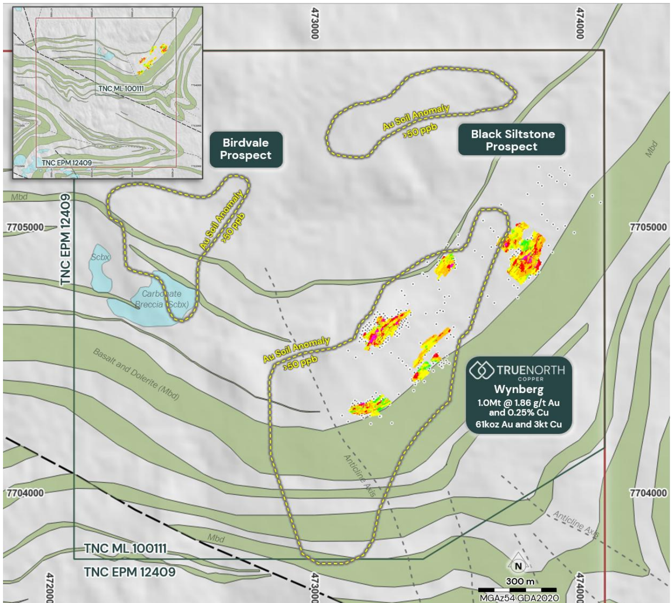
Figure 5. Local Structure and Geology
