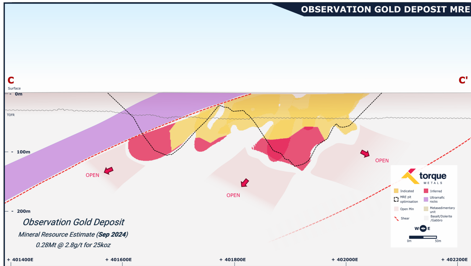
Figure 6 September 2024 Mineral Resource Estimate, Observation Deposit, E-W Section.
