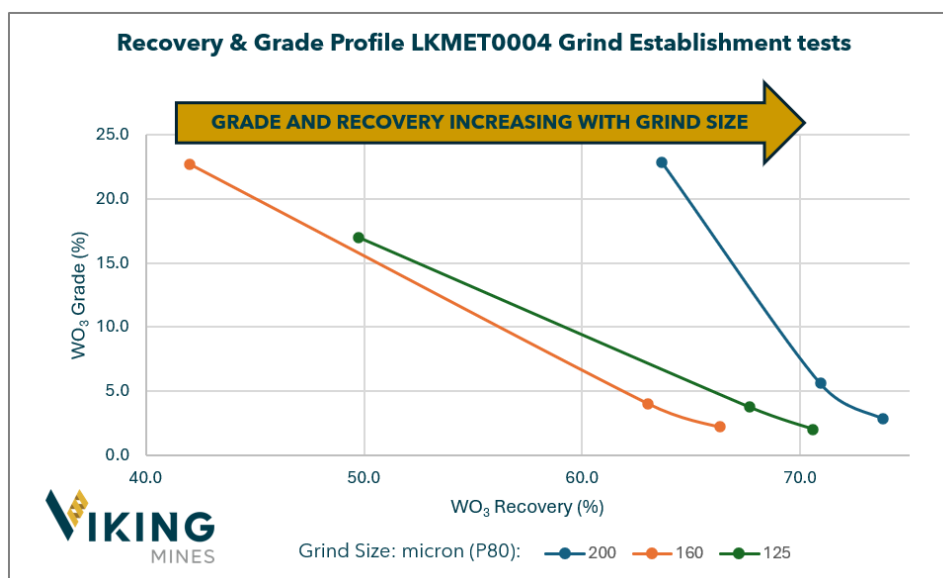
Figure 1; Graph showing results from three grind establishment tests conducted on the LKMET0004 sample. Increasing grade and recovery was achieved at the coarsest fraction (200 micron) indicating potential for higher recoveries and grades at coarser grind sizes yet to be tested.
