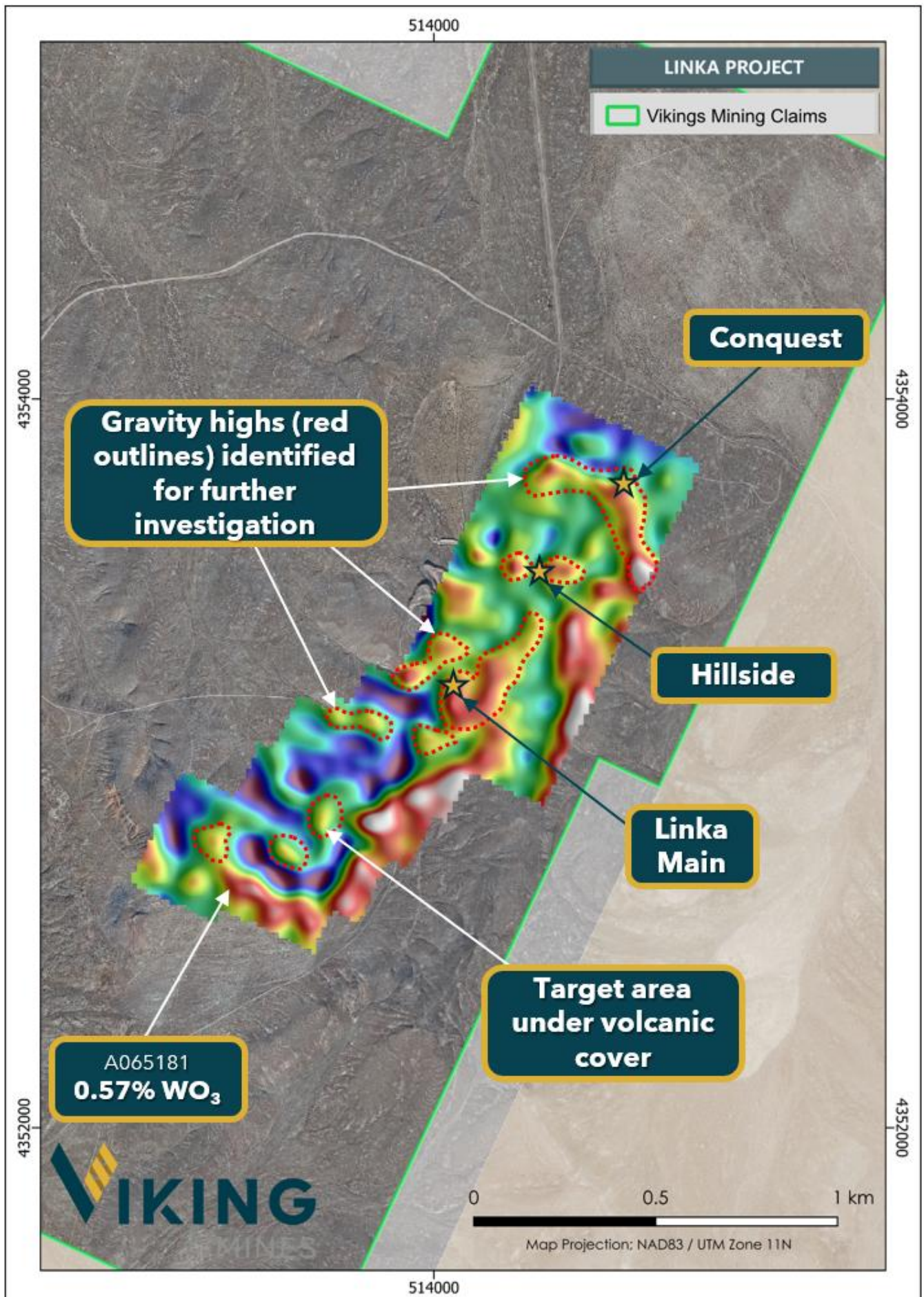
Figure 2; Map showing terrain corrected bouguer anomaly gravity image with Linka Main, Hillside and Conquest historic mines annotated and coincident with gravity highs.
