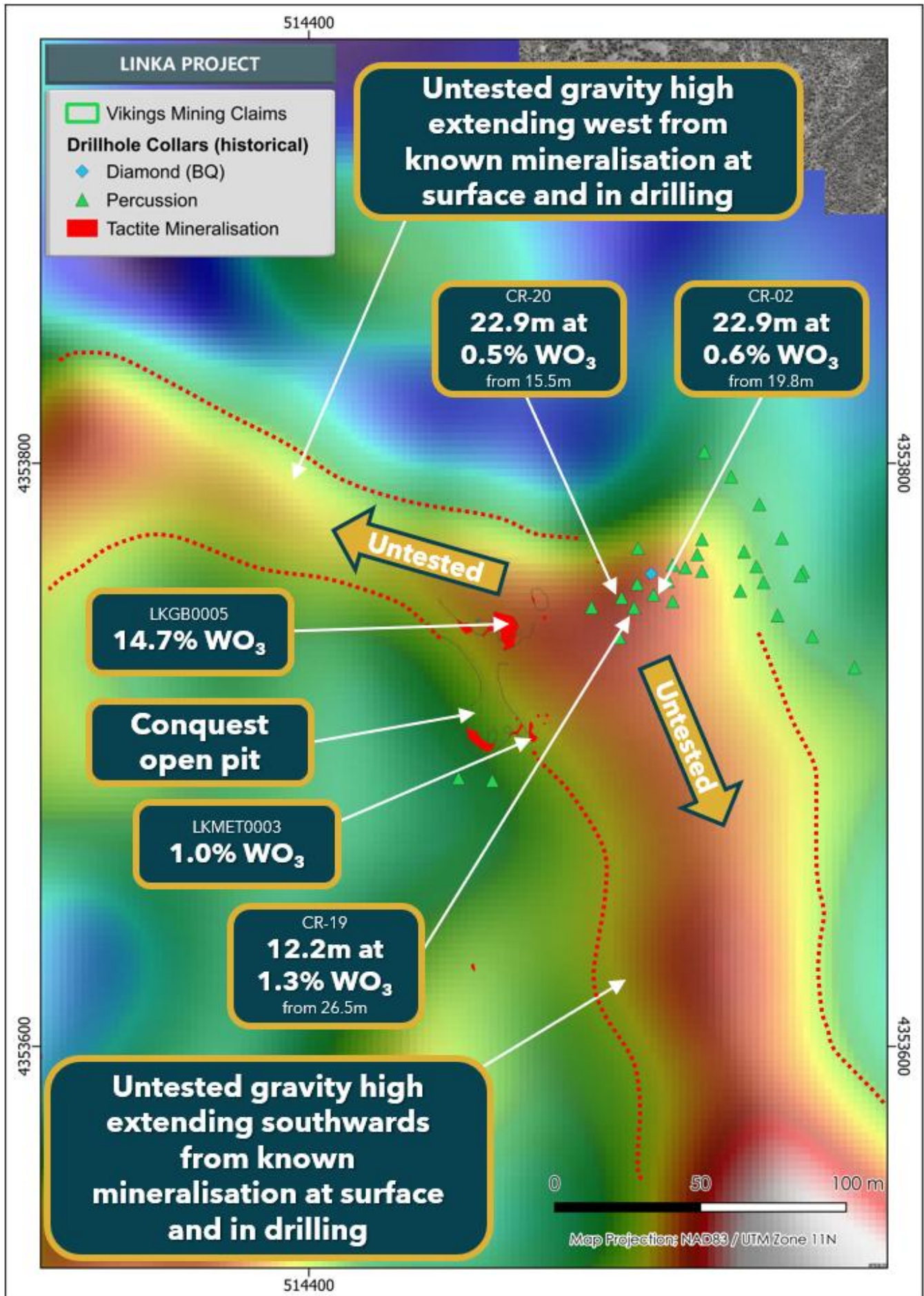
Figure 5; Map showing terrain corrected bouguer anomaly gravity image at Conquest with historic drillhole results and extensive untested gravity high to the south and west.
