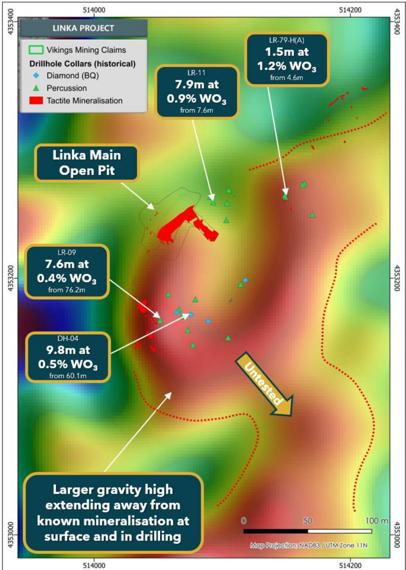
Figure 4; Map showing terrain corrected bouguer anomaly gravity image at Linka Main with historic drillhole results and extensive untested gravity high to the south.
