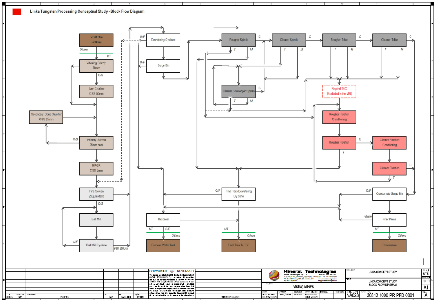
Figure 1; Block flow diagram illustrating the conceptual flowsheet design for the Linka Project conceptual processing study.
