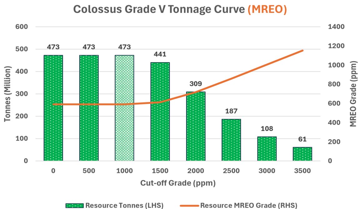
Figure 3: Colossus REE Project MREO grade-versus-tonnage curve, showing the variation in resource tonnage and average MREO grade across different TREO cut-off grades.
