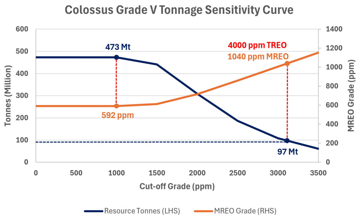
Figure 4: Colossus REE Project Grade Vs Tonnage Sensitivity Curve at different Cut-Offs, Dual Line Chart with Tonnage interpolated at 97Mt for grades at 4,000ppm Grade.
